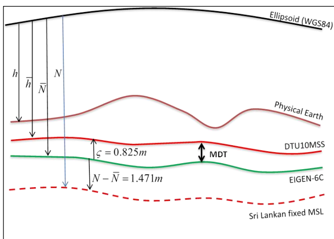
Fig. 3: Different vertical datums, and their variations over the Colombo tide gauge station
