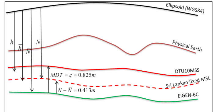
Fig. 5: variations of different vertical datums over Colombo tide gauge station after removing the GPS datum bias
