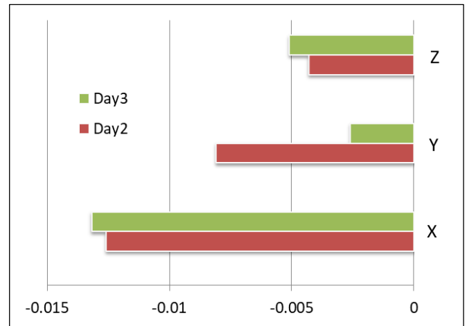
Fig. 4: Variation of X, Y, Z coordinates with respect to the day 1 solution (values in meters).
