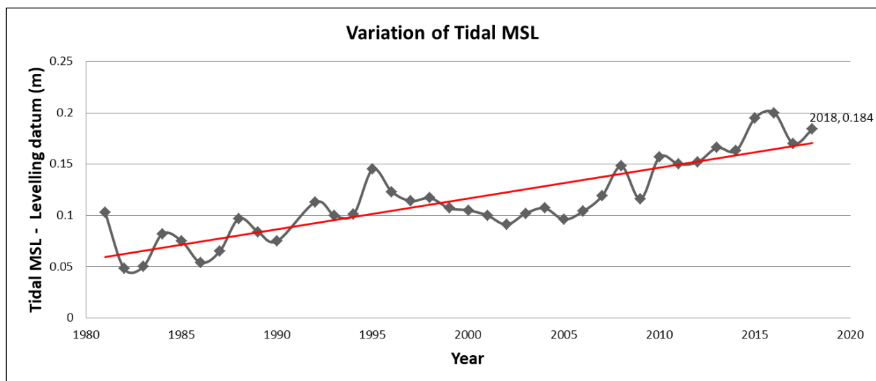
Fig. 2: Variation of Tidal MSL over the Levelling datum at Colombo Tide Gauge Station (From 1981-2018, 37 years)
