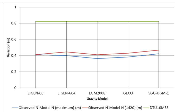
Fig. 6: Variation of observed-Model geoid undulations with respect to the DTU10MSS heights
