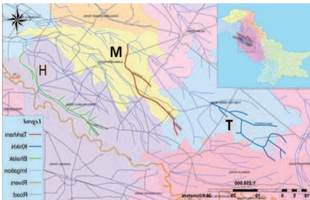
Figure 1: Location of the selected distributaries in the LCC East irrigation system
