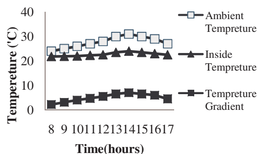
Figure 2: Temperature profile in charcoal cool-chamber and ambient condition.
