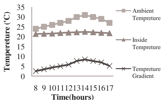
Figure 1: Temperature profile in sawdust cool-chamber and ambient condition
