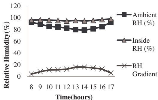
Figure 4: Relative humidity in charcoal cool-chamber and ambient condition
