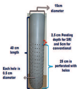
Plate 1: Field water tube specification and field installation view
