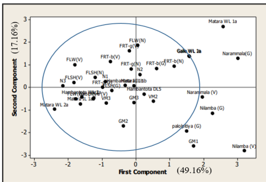
Figure 9: Score plot for leaf samples.
