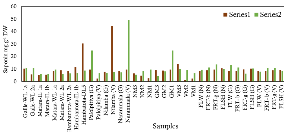
Figure 5: Comparison of saponin contents of leaves and bark of C. zeylanicum (Series 1: bark; Series 2: leaves).
