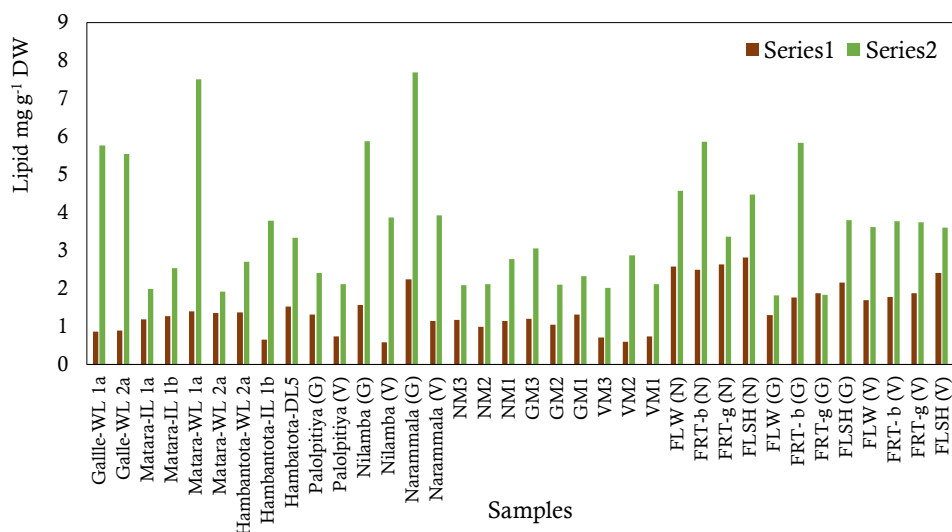
Figure 8: Comparison of lipid contents of leaves and bark of C. zeylanicum (Series 1: bark; Series 2: leaves).
