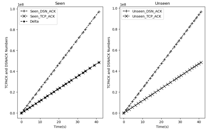
Figure 7. Experiment 1 - Link condition of seen subflow and unseen subflow are same (10Mbps of bandwidth and 10ms of latency). TCP_ACK and Delta series of Seen subflows is overlapped.
