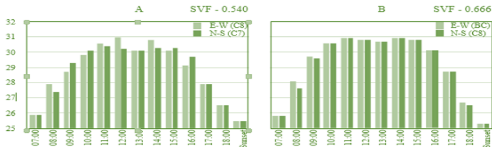
Figure 11. Orientation Analysis for similar SVFs for Street 1(N-S) and Street 2 (E-W)
