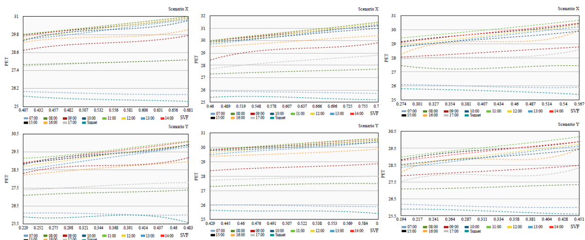
Figure 8. PET and SVF Correlation – Street 01 – Receptor A, Receptor B and Receptor C – Scenario X and Y
