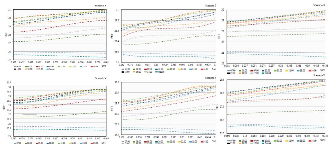
Figure 10. PET and SVF Correlation – Street 02 – Receptor A, Receptor B and Receptor C – Scenario X
