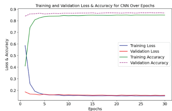
Figure 6 - Training and Validation Accuracy Over Epochs for "CNN" Model
