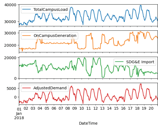
Figure 1 - Feature Variations Plot for 20 Days
