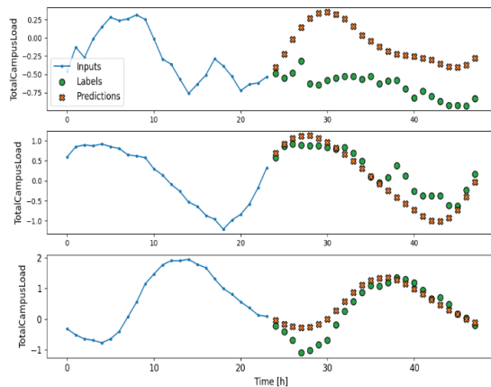
Figure 3 - Actual vs Predicted Plot for CNN Model
