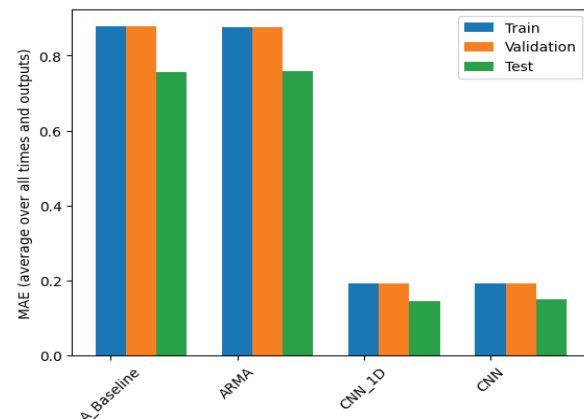
Figure 7 - MAE Values of all the Models
