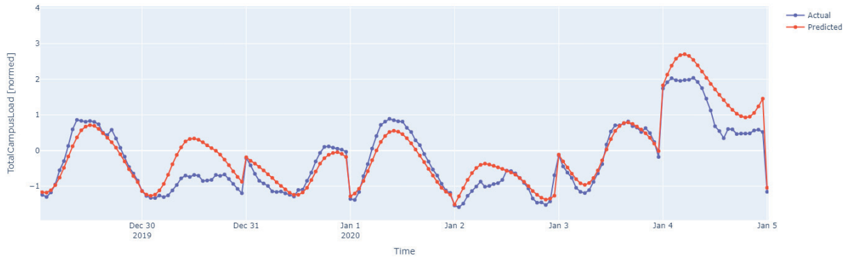
Figure 4 - Actual vs Predicted Data of Test Data Set for a Week
