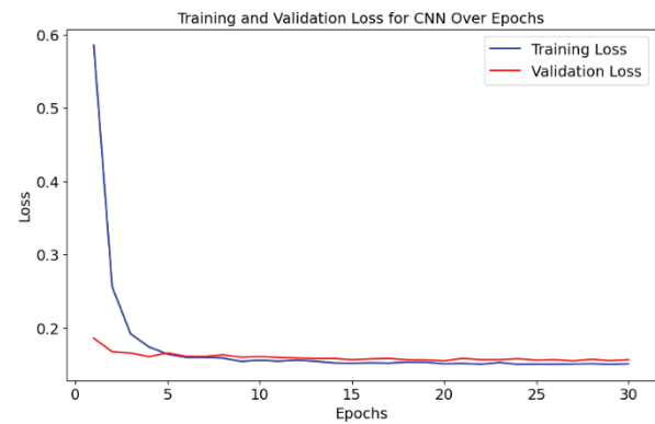
Figure 5 - Training and Validation Loss Over Epochs for "CNN" Model
