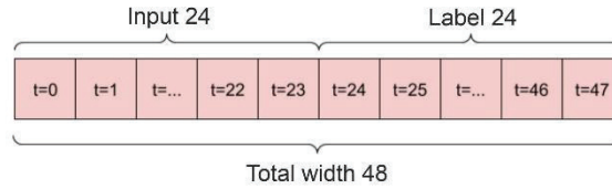
Figure 2 - Data Window with Input and Label Data Points
