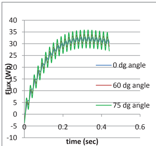
Figure 5 - Variation of core flux with secondary burden phase angle
