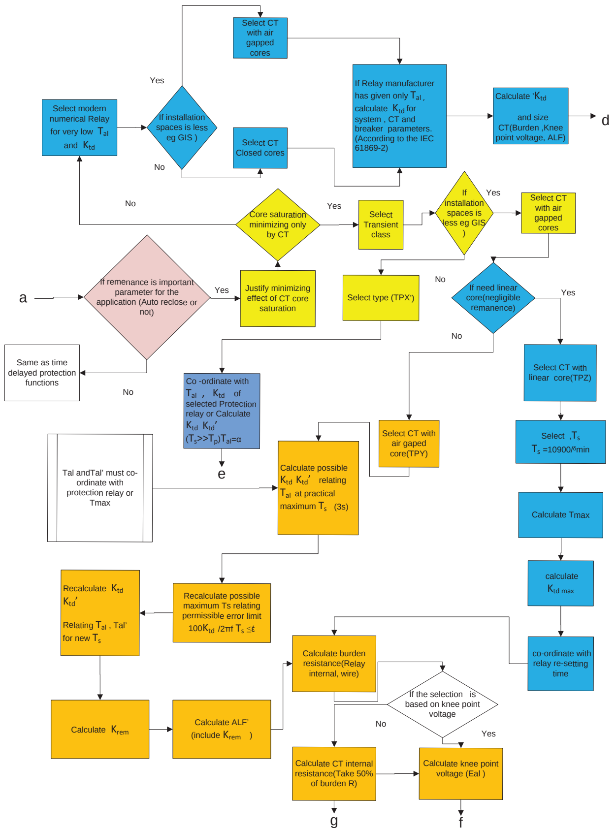
Figure 7 - Network and CT Parameters based CT Selection Criteria (continued on next page)
