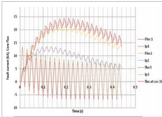
Figure 4 - Variation of Core Flux with T_2
