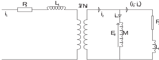
Figure 2 - Equivalent Circuit of a CT
