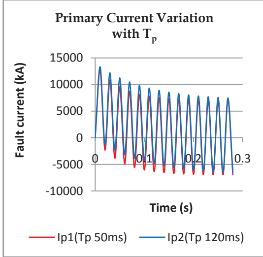
Figure 1 - Primary Current Variation with T_p
