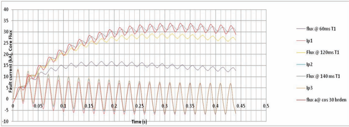
Figure 3 - Development of CT Core Flux with different TPs and a constant TS (= 1000ms)
