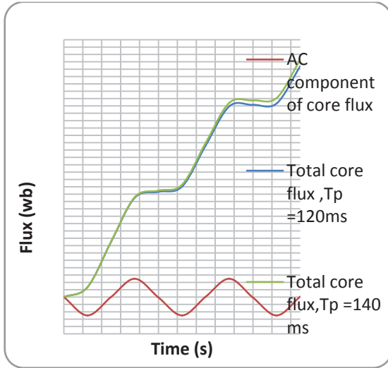
Figure 6 - AC Flux Component and Total Flux Development of the CT Core.
