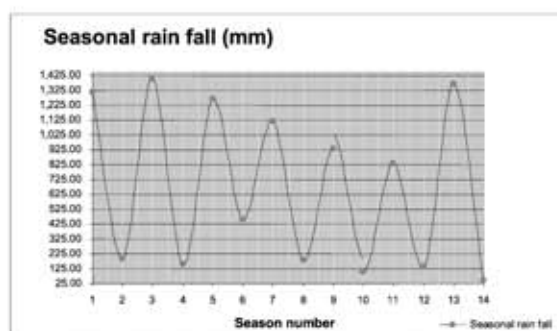
Fig 4.1 Average seasonal rain fall
