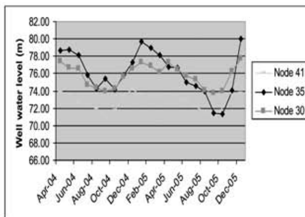
Fig. 4.3 Monthly Groundwater Level Fluctuation
