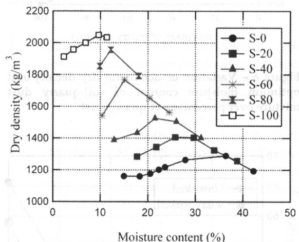
Figure 5 - Compaction curves for soil-quarry dust mixtures
