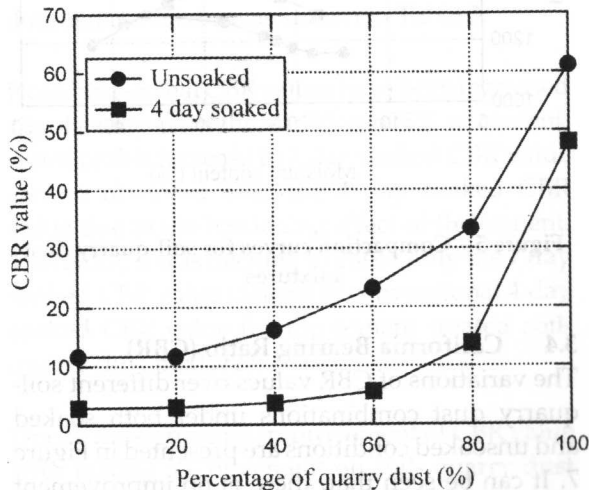
Figure 7 - Variation of CBR value for different soil-quarry dust mixtures
