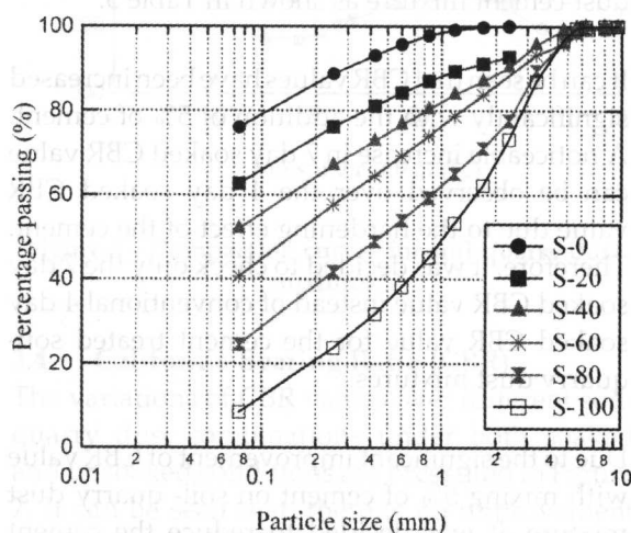
Figure 2 - Particle size distribution of soil-quarry dust mixtures
