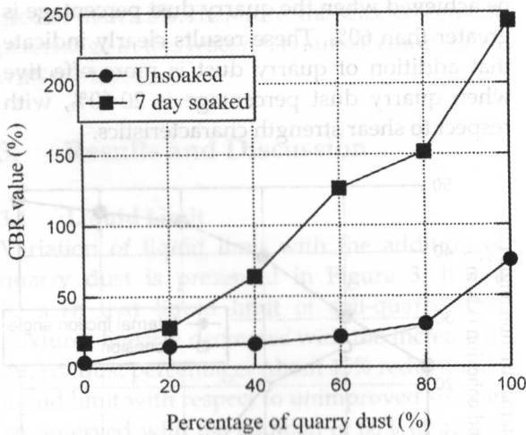
Figure 8 - Variation of CBR value for different soil-quarry dust mixtures with the addition of 2% of cement
