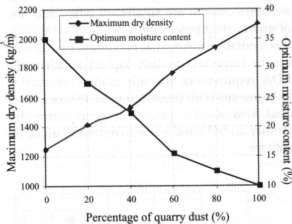
Figure 6 - Variation of maximum dry density and optimum moisture content of soil-quarry dust mixture over percentage of quarry dust
