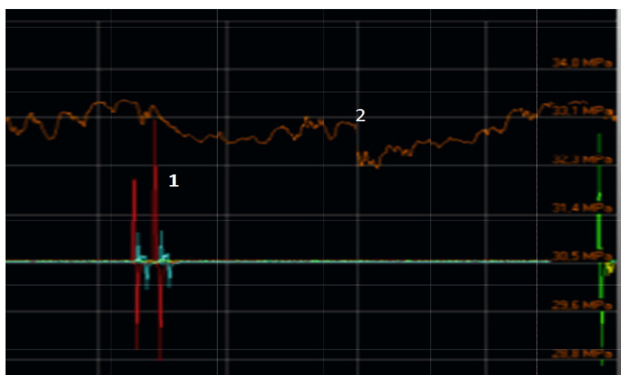
Fig. 4. Current characteristics of the injector coils (1) and the pressure in the "fuel rail" (2). Source: Own study
