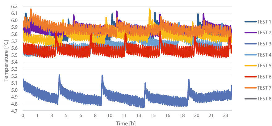
Fig. 8. Average test temperatures (own study)
