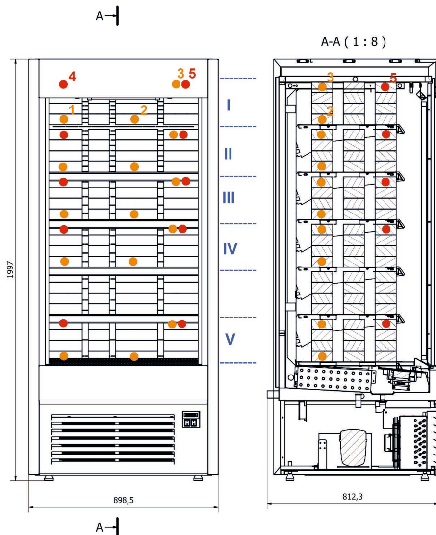
Fig. 2. VARNA refrigerated display rack with glazed sides, marked with measurement packages (I – first level, II – second level, III – third level, IV – fourth level, V – fifth level) (own study)
