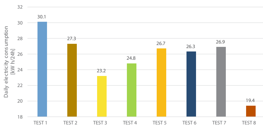
Fig. 9. Electric energy usage (own study)
