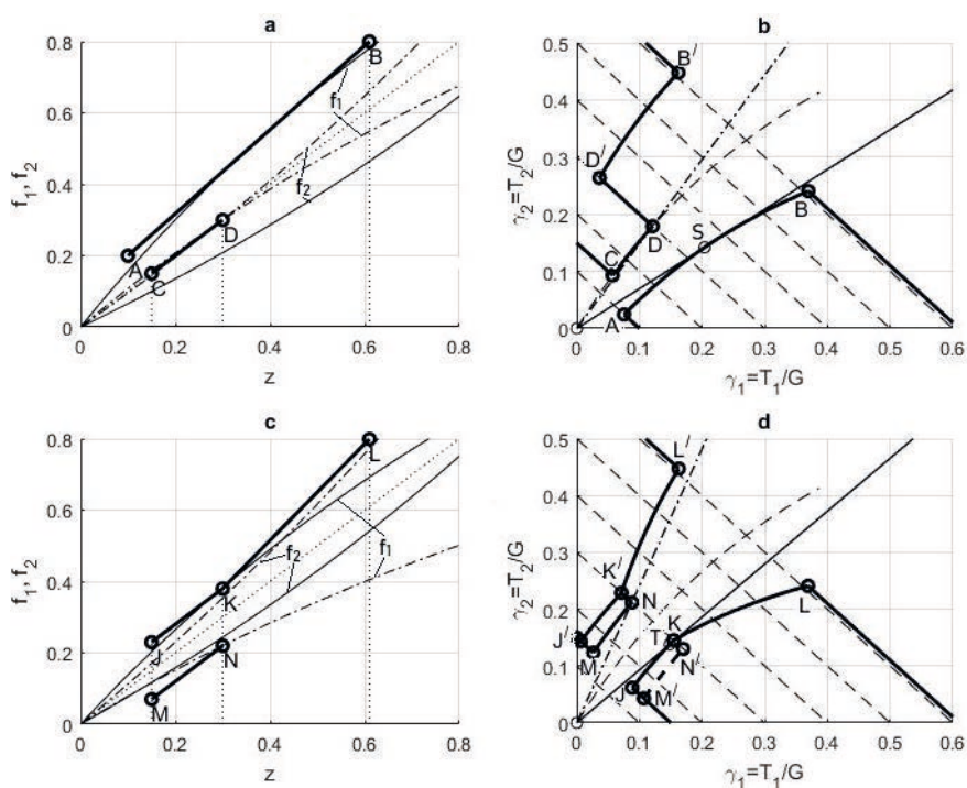
Fig. 4. Determination of parameters of constant brake force distribution between unladen trailer axles with parameters: m=7700\text{ kg} , L=5.15\text{ m} , b=1.85\text{ m} , h=1.08\text{ m} , L_2=1.2\text{ m} , l_{2,1}=0.62\text{ m} , l_{2,2}=0.58\text{ m} , h_i=0.54\text{ m} : a and c – limit values of adhesion utilized rates, b and d – limit values of braking distribution between vehicle axles
