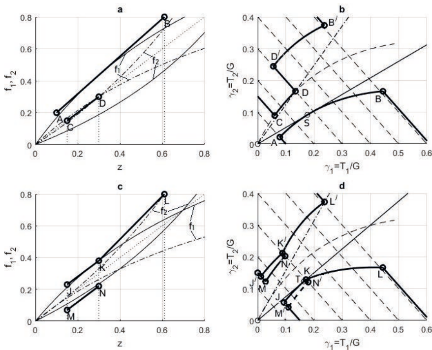
Fig. 3. Determination of parameters of constant brake-force distribution between laden trailer axles with parameters: m=24\,000\text{ kg} , L=5.15\text{ m} , b=1.85\text{ m} , h=1.8\text{ m} , L_2=1.2\text{ m} , l_{2,1}=0.62\text{ m} , l_{2,2}=0.58\text{ m} , h_i=0.54\text{ m} : a and c – limit values of adhesion utilized rates, b and d – limit values of braking distribution between vehicle axles
