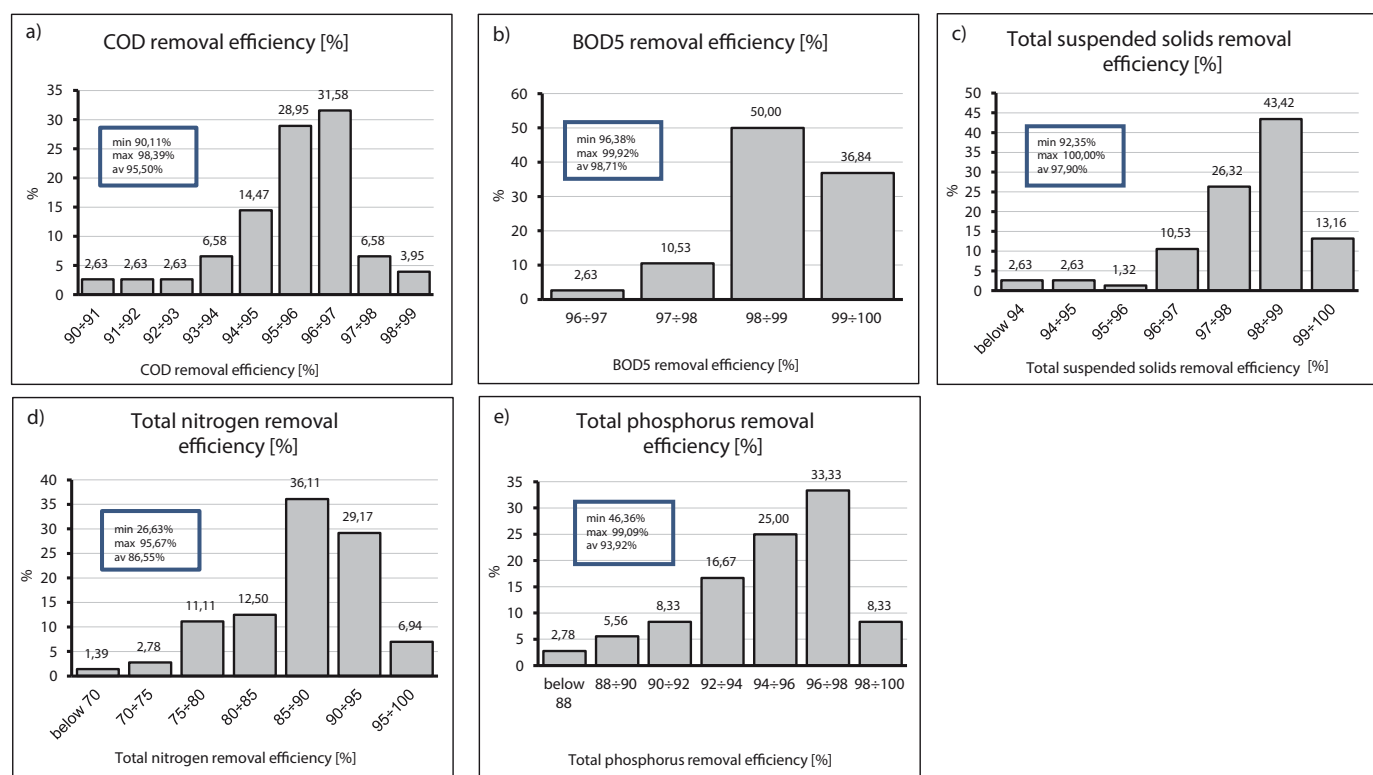
Fig. 2. Histograms representing sewage treatment plant efficiency in relation to: a) COD, b) BOD5, c) total suspended solids, d) total nitrogen, e) total phosphorus (Wójcicka, Heidrich, 2020)
