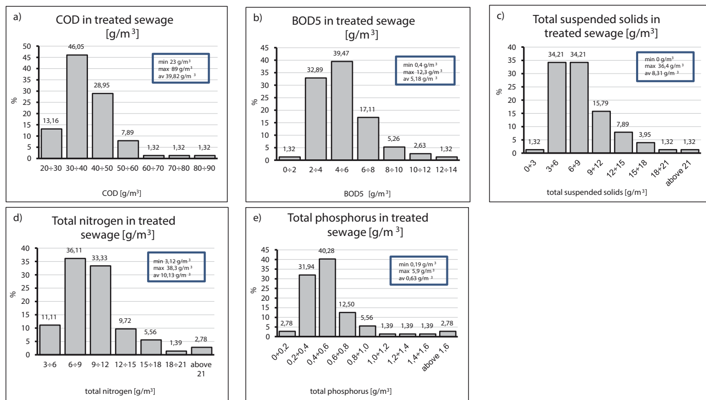
Fig. 1. Histograms representing contaminant concentrations in municipal sewage treatment plant effluent, based on actual data: a) COD, b) BOD5, c) total suspended solids, d) total nitrogen, e) total phosphorus (Wójcicka, Heidrich, 2020)
