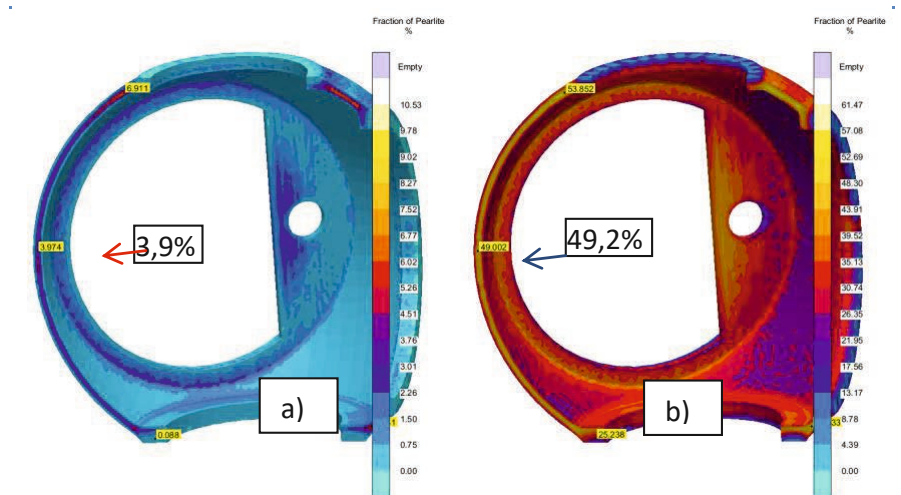
Fig. 2. Pearlite distribution in the cross section of an 11 tonne weighing rotor hub for C = 3.8 and Si = 2.0 and the spheroidising treatment process of: a) very high effectiveness and b) low effectiveness (author's work)
