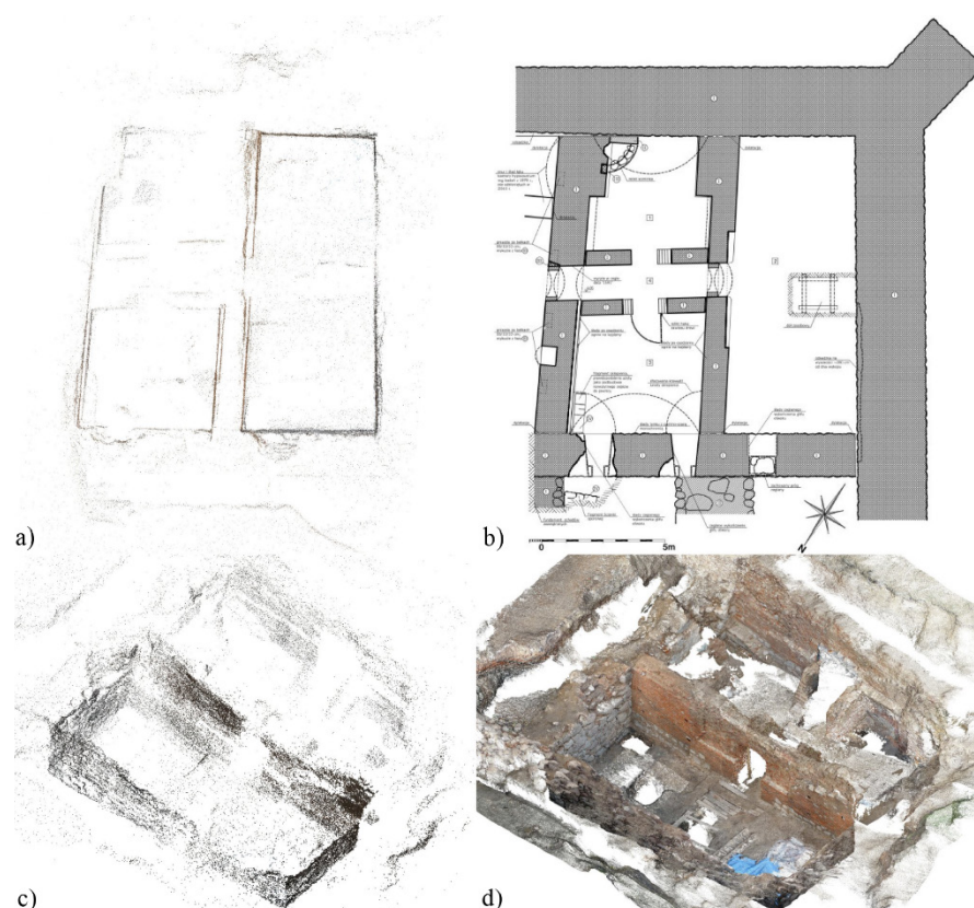
Fig. 1. Kruszwica, Castle, a fragment of the palace cellars excavated during archaeological works in 2010 (Małachowicz and Karnicki, 2010); a) photogrammetric reconstruction (Microsoft PhotoSynth) of the basement projection; b) inventory drawing with chronological stratification of the walls; c) isometric view of the excavation area – a point cloud (about 65,000 points) made from 136 photos (4 Mpix) created in 2010 with Microsoft PhotoSynth, calculation time was approx. 4 hours; d) isometric view of the place – point cloud approx. 4.5 million points, an comparable set of photographs, created in 2017 with Agisoft Metashape software, calculation time was approx. 10 min
