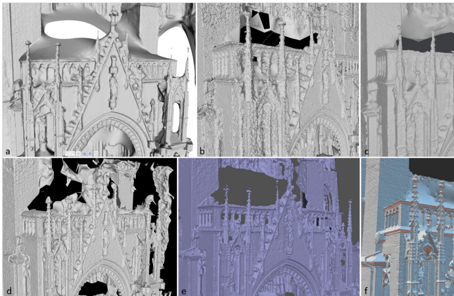
Fig. 4. Comparative comparison of texture-free meshes to judge the quality of geometry representation – all models are shown in the highest quality offered by the software: a) Autodesk ReCap Photo – good representation of wall planes but some simplifications in the perforation area; b) Meshroom, mesh before optimisation, good visible detail and significant noise; c) Meshroom, mesh after denoising process, visible loss of geometry detail; d) 3DF Zephyr Free, good quality mesh with good detailing; e) Agisoft Metashape, a high-quality mesh with a good detailing and perforation coverage – at the uprights there are some detailing problems but captured profiles and wall material texture are recognisable; f) RealityCapture, perfect reproduction of geometry and complexity of the detail where small-size elements are also shown
