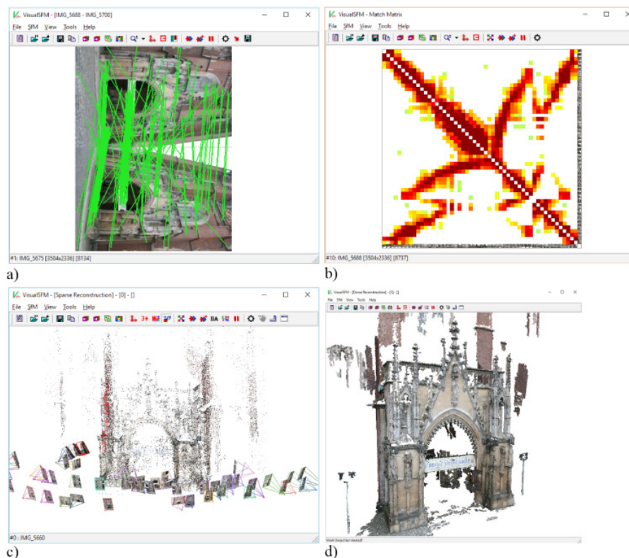
Fig. 2. Illustration of following photo reconstruction steps – VisualSFM (Changchang Wu, 2020); reference site – main western portal of St. John the Baptist Cathedral in Wrocław: a) visualisation of connections between recognised characteristic points of two matching images; b) matrix which shows relations grade between individual frames (bronze – best fit); c) spatial location of cameras stands and a sparse point cloud of characteristic points of the shots; d) dense point cloud obtained using CMVS+PMVS modules (approx. 4 million points, calculation time 3 hours, 2015)
