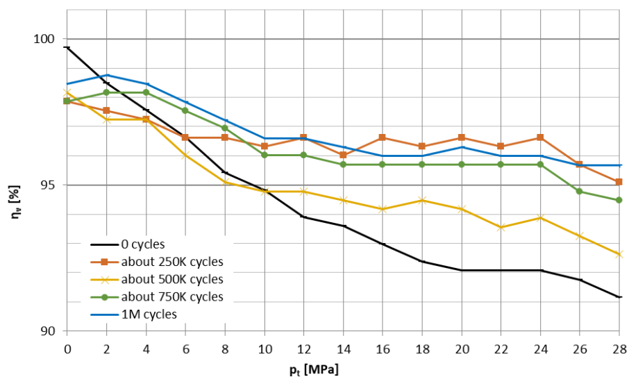
Fig. 5. Comparison of the volumetric efficiency during the durability test for the speed of 1000 rpm (source: own compilation)
