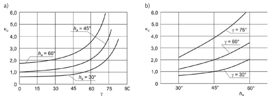
Fig. 2a. The value of the facade shading measured from the overhanging elements, with respect to the location of the building relative to the four compass points (angle h_p ), assuming different values of solar angular height h_a
