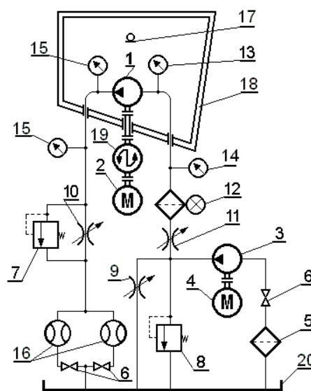
Fig. 2. Scheme of the measurement stand: 1 – tested gear pump; 2 – DC drive motor; 3 – feed pump; 4 – AC motor; 5 – suction filter; 6 – shut-off valve; 7, 8 – safety valves; 9, 10, 11 – stop valves; 12 – flood filter; 13, 14 – vacuum/pressure gauges; 15 – manometer; 16 – flow meter; 17 – measuring microphone; 18 – acoustic chamber; 19 – torque gauge; 20 – tank (source: Osiński, 2013)
