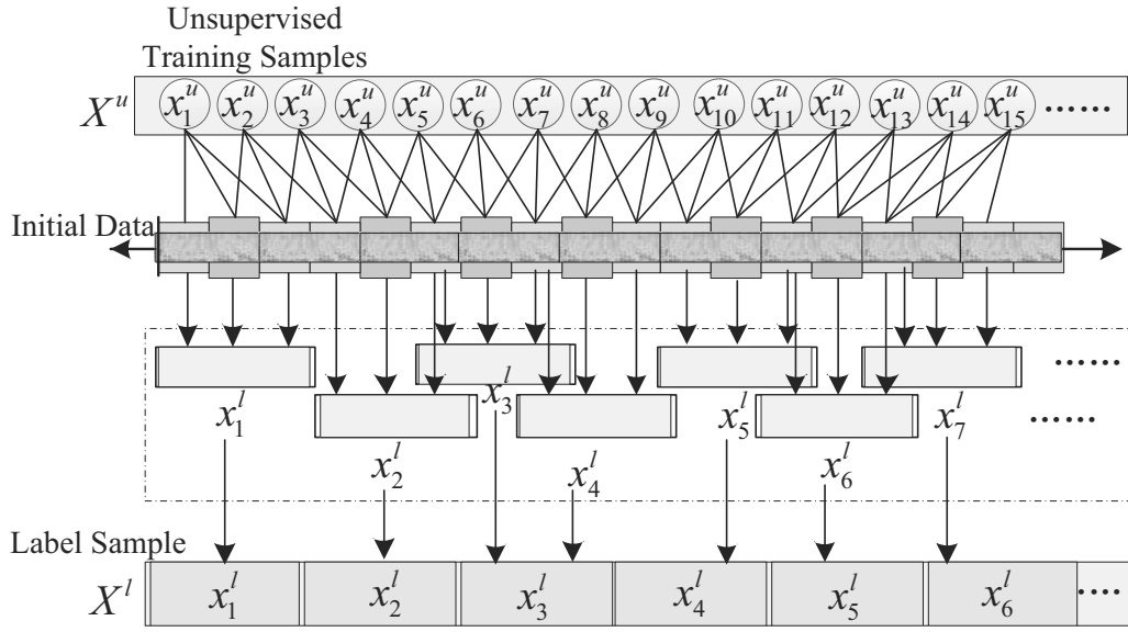
Fig. 2. Construction of training samples with dynamic time.
