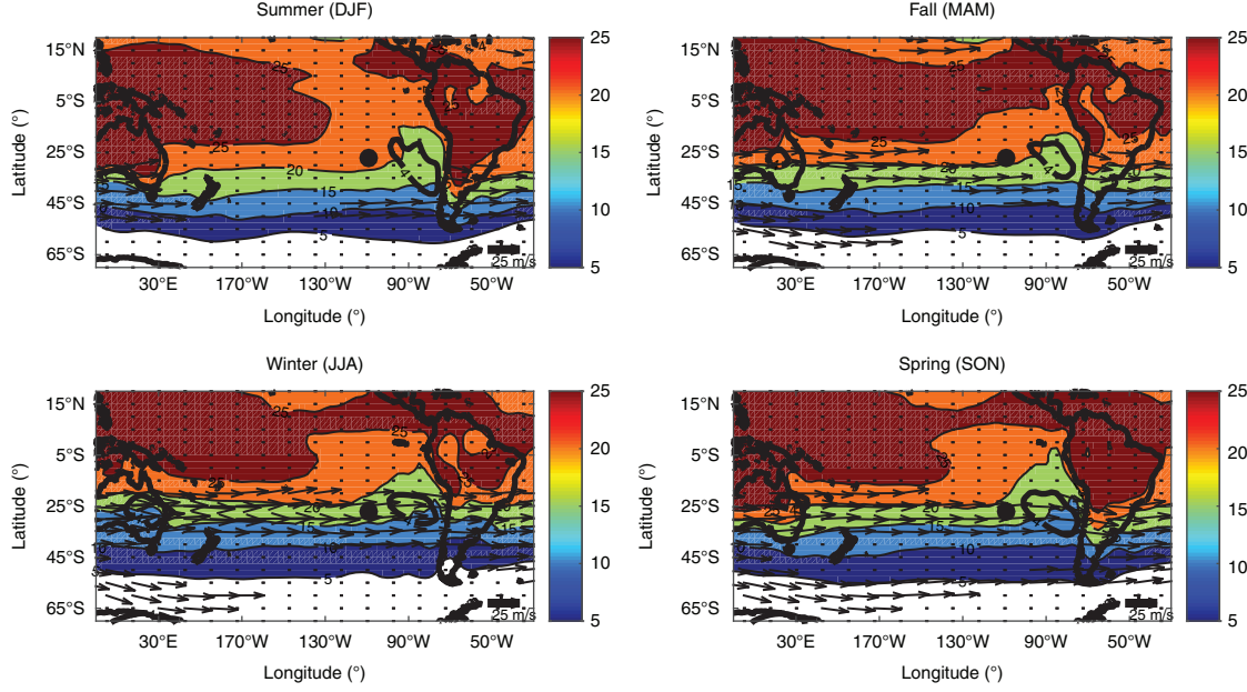
Fig. 4. Subtropical jet stream, surface temperature and subsidence in the Pacific along the year. Arrows show wind velocity in excess of 25 m/s at 200 hPa. Surface temperatures in °C (at 1000 hPa) are also shown. The area with omega velocities in excess of 4 hPa/s, that is, regions of prevailing subsidence are indicated with a black line. The black dot indicates the location of Rapa Nui. Data: NCEP/NCAR Reanalysis.
