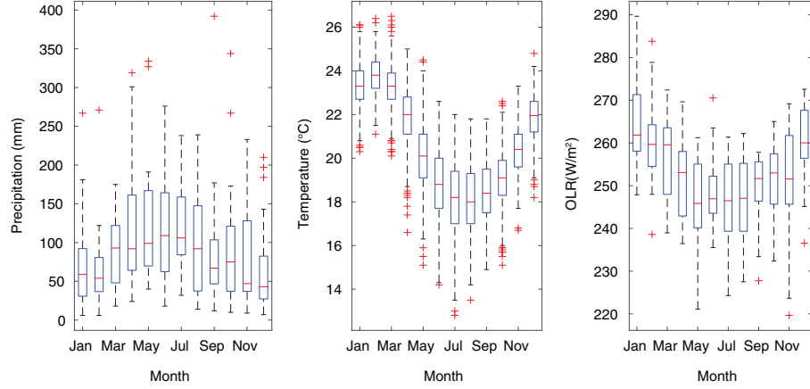
Fig. 6. Precipitation (in mm/month, left panel), surface temperature (in ^{\circ}\text{C} , middle panel) and outgoing long-wave radiation (OLR, in \text{W/m}^2 , right panel) climatologies over Rapa Nui for the period 1994–2014. Precipitation and temperature were obtained from the Chilean Weather Office. OLR values obtained from NCEP/NCAR reanalysis. Data are presented as box plots: the central mark in the box indicates the median of the distribution, the edges of the box are the 25th and 75th percentiles, the whiskers extend to the most extreme data points not considered outliers, and outliers are plotted individually (red crosses).
