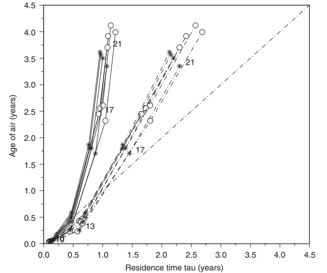
Fig. 11. Simulated vertical profiles of age of air vs. residence time \tau of aerosols. Four levels are represented, at approximately 10, 13, 17 and 21 km (cf. labels). Full lines: simulation with beryllium sedimentation; dashed–dotted lines: simulation without sedimentation. Circles underline southern high-latitude profiles (approx. 85^\circ\text{S} to 57^\circ\text{S} ); stars underline northern high-latitude profiles (approx. 85^\circ\text{N} to 57^\circ\text{N} ).
