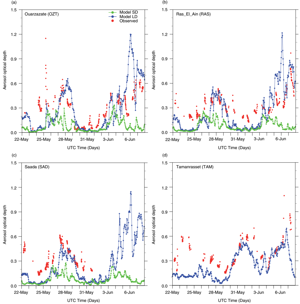
Fig. 4. Plots of the column AOD time series for the period of the SAMUM-I experiment: observation at 0.551\ \mu\text{m} (red) from four AERONET stations and simulation at 0.6\ \mu\text{m} in the LD (blue) and SD (green) at (a) Ouarzazate (OZT), (b) Ras-Al-Ain (RAS), (c) Saada (SAD), and (d) Tamanrasset (TAM). The geographical coordinates of the AERONET stations are provided in Table 1. AERONET level 1.5 data are used. TAM is beyond SD, and therefore TAM AERONET AOD cannot be compared with the AOD simulated in SD.
