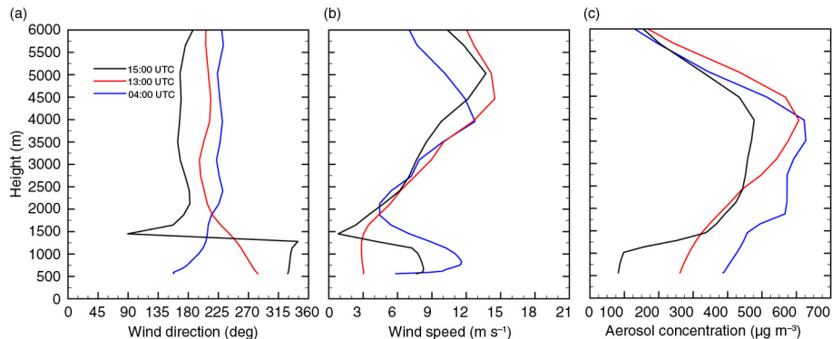
Fig. 12. Vertical profiles of (a) wind direction (degrees), (b) wind speed (m s -1 ), (c) aerosol concentration (µg m -3 ) on 7 June 2006 at 04:00, 13:00 and 15:00 UTC in the location of 6.3°W, 33.5°N as indicated by the red arrow in Fig. 11f.
