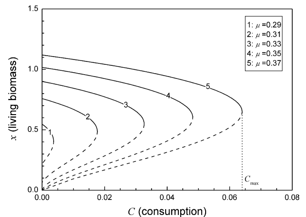
Fig. 9. The equilibrium state of the living biomass as a function of fixed consumption C . For each moisture index \mu , there exists a maximum value of consumption, C_{\max} , and no grassland is maintained as C > C_{\max} (in this figure C_{\max} for curve 5 is marked).
