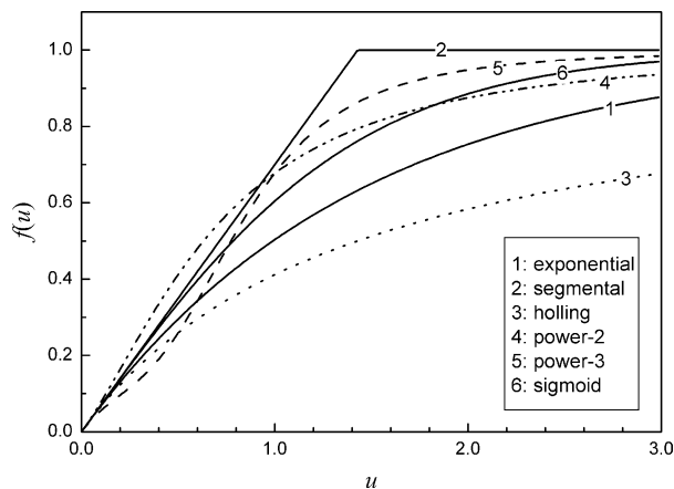
Fig. 3. The sketch of the different functions f(\varepsilon, u) defined in eqs (31)–(36) with \varepsilon = 0.7 . For curves 4 and 5 the functional coefficients a_{22} = 2.0 , a_{32} = 1.0 and a_{33} = 4.0 .
