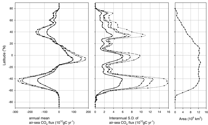
Fig 5. Latitudinal profiles of annual mean air-sea CO 2 exchange and the interannual standard deviation induced by k variations computed using NCEP winds, Takahashi \Delta p CO 2 data and different k - U_{10} parametrizations: k_{LM86_i} , thick full curve; k_{W92_i} , thin full curve; k_{W92_{av}} , dashed curve; k_{WM99_i} , dotted curve. The panel to the right shows the zonal distribution of ocean surface area.
