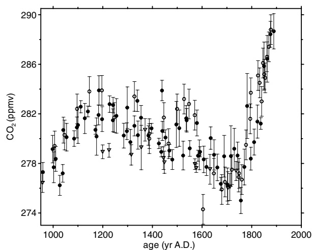
Fig. 1. Full circles: CO 2 data from DML. Open triangles: New measurements on the South Pole ice core. Both records were measured with dry extraction (mean of six samples; error bars, 1 \sigma of the mean). Open circles: Law Dome data (Etheridge et al., 1996).
