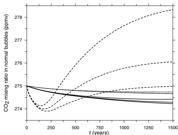
Fig 3. Calculation of the CO 2 concentrations of air enclosed in normal bubbles with the boundary conditions explained in the text, t = 0 is at close-off. For every site, three calculations were made with different initial CO 2 concentrations in the microbubbles of 275, 500 and 1000 ppmv. The corresponding equilibrium concentrations (if all air from the microbubbles and normal bubbles is mixed up) are 275, 276.1 and 278.6 ppmv, respectively. Dashed curves: calculations for Law Dome DSS (mean temperature -22^{\circ}\text{C} ). Full curves: calculations for DML ( -44.6^{\circ}\text{C} ). Dotted curves: calculations for the South Pole ( -51^{\circ}\text{C} ).
