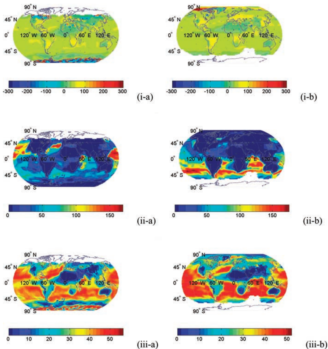
Fig 2. Global distribution of percentage differences ( \Delta F in %) in the reference aerosol forcings (Fig. 1) induced by increasing the RH by 10% of its reference value for (a) January and (b) July. The aerosol forcings are explained in Fig. 1.
