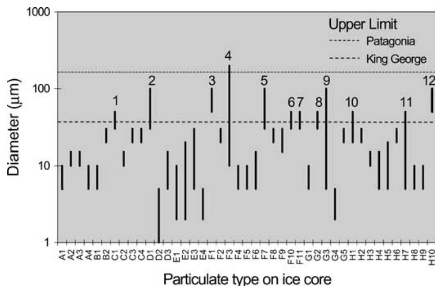
Fig 3. Range of diameters of insoluble particles found in the Lange ice core. Dashed lines indicate Patagonian and King George Island upper limits.
