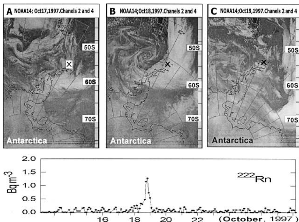
Fig 1. Eastward movement of a cyclonic system between South America and the Antarctic Peninsula with simultaneous increase of ^{222}\text{Rn} activity concentration. A, B and C indicate a 3-day satellite image acquisition at the Brazilian Antarctic Station. X marks the location of the sampling station.
