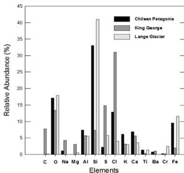
Fig 4. Relative abundance of insoluble particles in the Lange Glacier ice core and air at King George Island and Chilean Patagonia.
