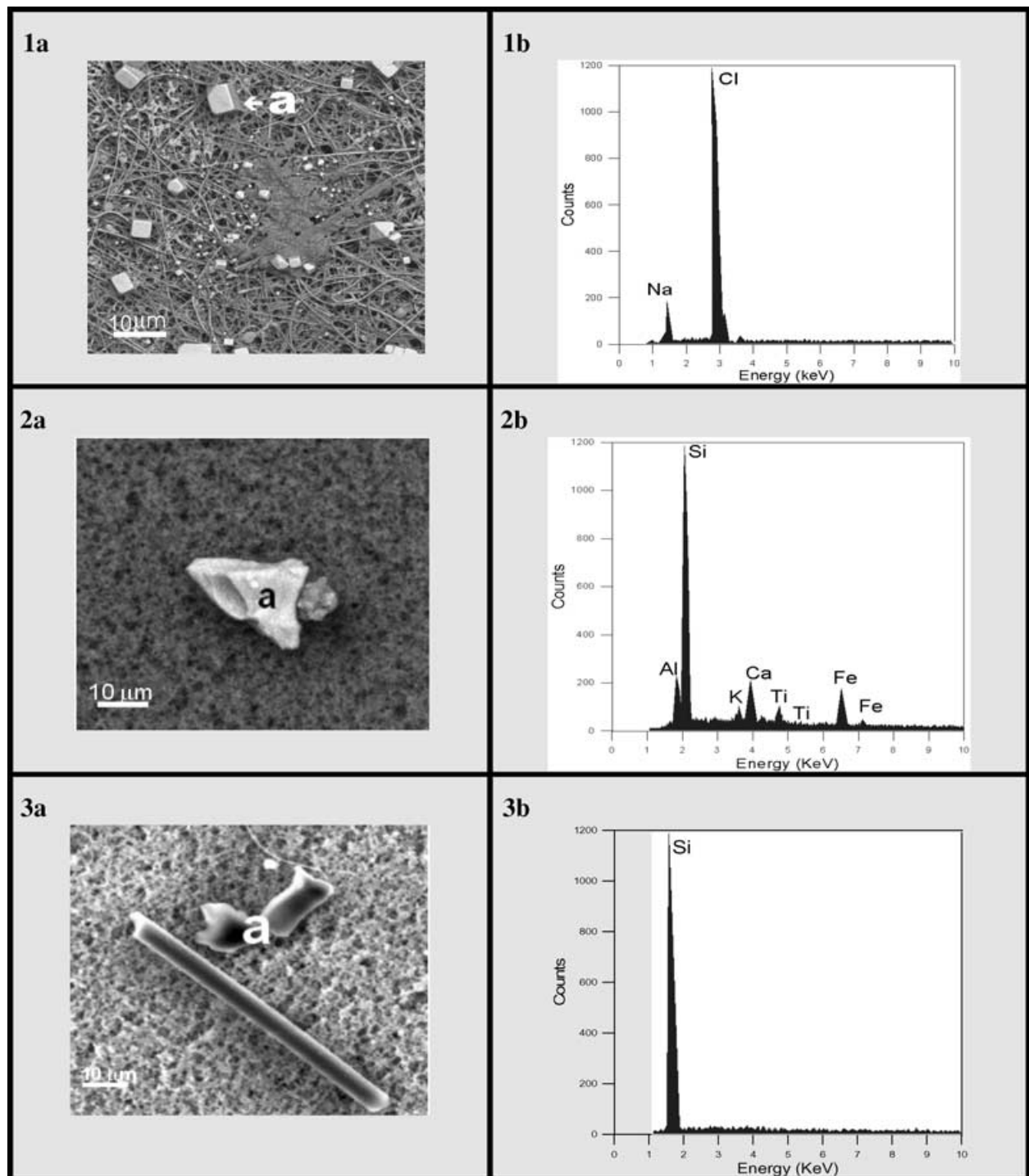
Fig 2. Morphology and corresponding spectrum of individual elemental composition for predominant insoluble particles in King George Island (1a and 1b), Chilean Patagonia (2a and 2b) and the Lange Glacier (3a and 3b). The "a" in the photographs indicates the electron target location.
