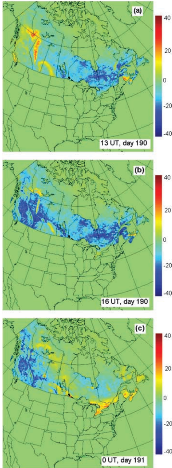
Fig 15. The evolution of the spatial distribution of the NEP fluxes for (a) 13 UT, day 190, (b) 16 UT, day 190 and (c) 0 UT, day 191. The contours are in units of 10^{-8} \text{ kg C m}^{-2} \text{ s}^{-1} . Positive indicates a flux of CO 2 from the biosphere to the atmosphere.
