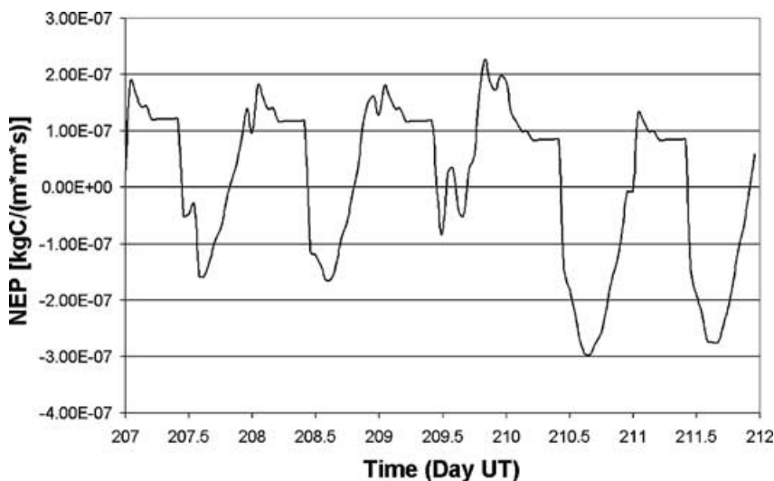
Fig 10. The evolution of the BEPS NEP flux at Fraserdale. Positive indicates a flux of \text{CO}_2 from the biosphere to the atmosphere.
