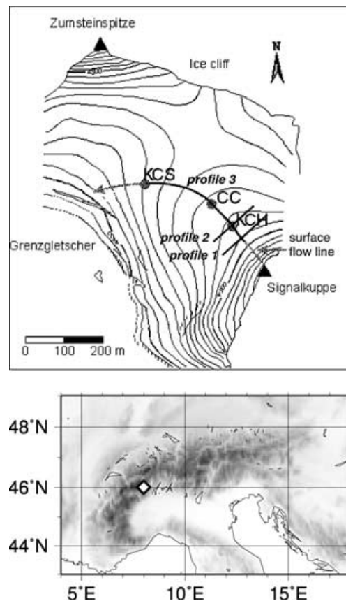
Fig. 1. Surface topography of southern Colle Gnifetti flank showing the location of deep ice core positions and GPR profiles 1–3. Contour lines refer to 10 m altitude steps. The white diamond in the lower topographic map indicates the location of the study area in the European Alps.
