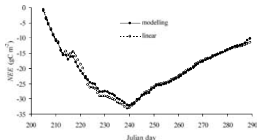
Fig. 10. Cumulated NEE , estimated by two methods of missing data in-filling: (1) process-based modelling and (2) linear interpolations.
