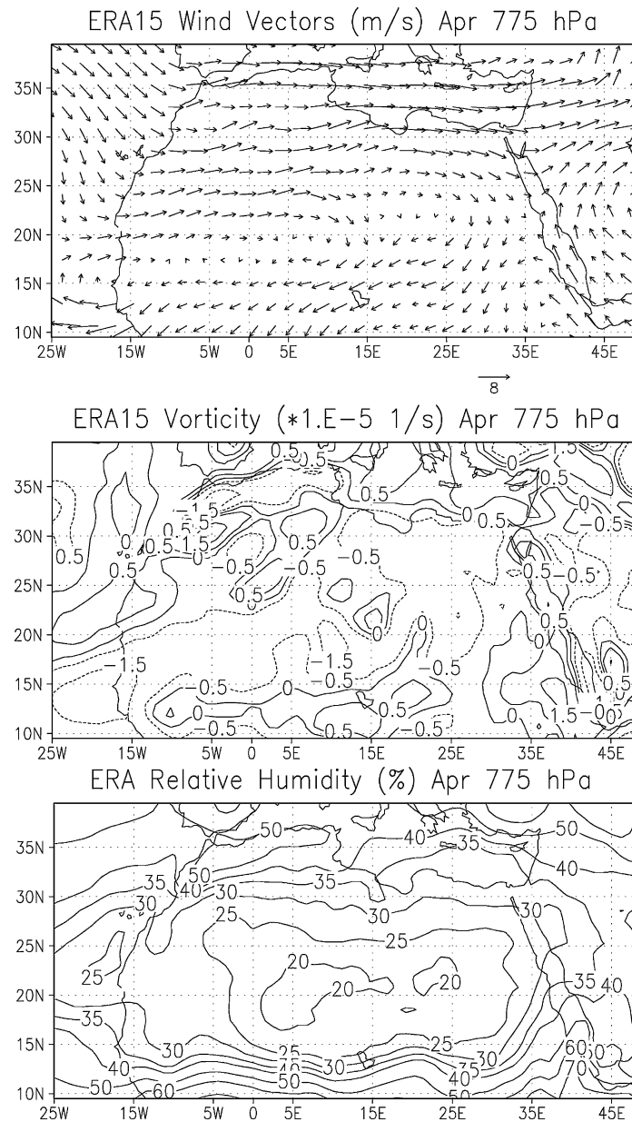
Fig. 5. The 2D distribution of the average wind vectors (top panel), the average value of vorticity (middle panel) and the average value of relative humidity (bottom panel) for the month of April in the years from 1979 to 1993 at the pressure level 775 hPa. The ERA15 reanalysis data were used.
