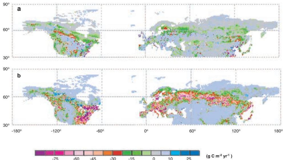
Fig. 7. A comparison of the spatial patterns of estimated annual changes in vegetation carbon storage during the 1980s and 1990s between (a) the TEM 5.0 S3 simulation and (b) the analysis of Myneni et al. (2001) based on remote sensing data. The TEM 5.0 estimates are based on differences that occurred from 1980 through 1995. The remote sensing estimates are aggregated into 0.5° × 0.5° resolution based on 0.25° × 0.25° resolution data (Myneni et al., 2001) to compare to the TEM estimates and represent differences in vegetation carbon storage between the period from 1980 to 1982 period and the period from 1995 to 1999. For easy of comparison, the color scheme used in this figure is similar to the one used in Myneni et al. (2001). Positive values in the plot represent sources of CO 2 to the atmosphere, while negative values represent sinks of CO 2 into terrestrial ecosystems.
