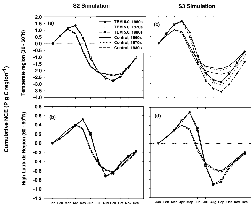
Fig. 5. The cumulative difference between NCE during the 1960s, 1970s and 1980s as estimated by the S2 simulations of TEM 5.0 and TEM 4.2 (control) for terrestrial ecosystems (a) between 30 and 60° N and (b) between 60 and 90° N; and by the S3 simulations of TEM 5.0 and TEM 4.2 for terrestrial ecosystems (c) between 30 and 60° N and (d) between 60 and 90° N. Lines with symbols indicate the results associated with soil thermal effects in TEM 5.0, and lines without symbols indicate results of the control simulation.
