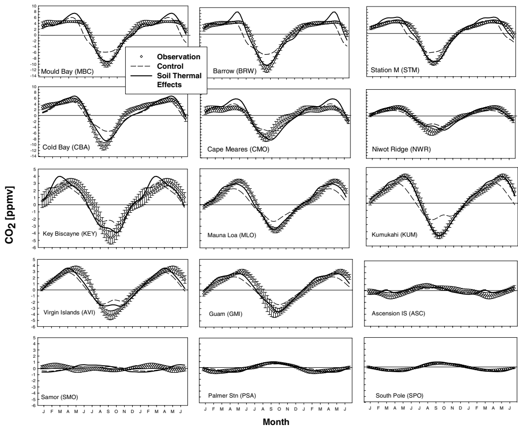
Fig. 4. Comparisons between the observed seasonal cycle of \text{CO}_2 and simulated seasonal cycle for 15 monitoring stations of the NOAA/CMDL network. The mean and standard deviation from 1982 to 1995 are shown for the observed data. The simulated \text{CO}_2 concentrations were estimated by providing the monthly NCE estimates of the TEM 5.0 simulation (soil thermal effects, solid line) and the TEM 4.2 simulation (control, dashed line) to the Model of Atmosphere and Transport Chemistry (MATCH). The first 6 months of each cycle are displayed twice to reveal the annual variation more clearly.
