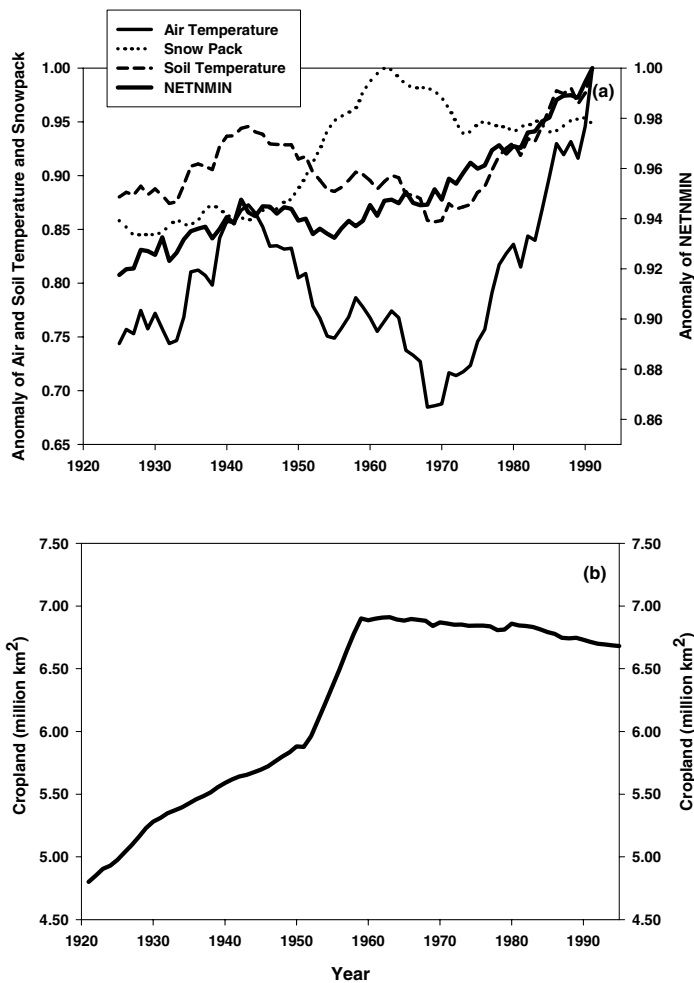
Fig. 8. Anomaly of air temperature, simulated snow pack, soil temperature and net nitrogen mineralization (NETNMIN) with TEM 5.0; the annual values were normalized to the range 0–1 and the data shown as 10 yr running mean (a) and land use (cropland) areas in extra-tropics of the Northern Hemisphere from 1920 to 1995 (b).
