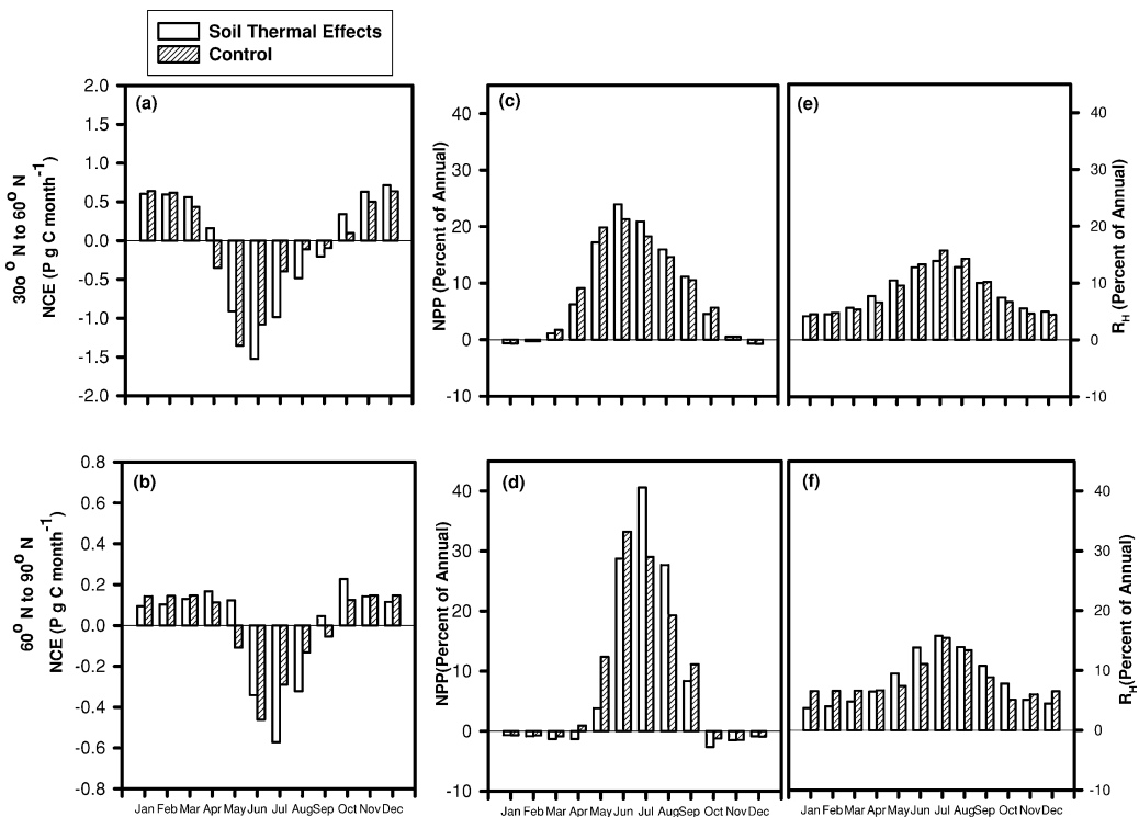
Fig. 3. Monthly simulated net carbon exchange (NCE, left panels) and monthly relative net primary production (NPP, center panels) and heterotrophic respiration ( R_H , right panels) as estimated by TEM 5.0 and its control simulations for 30–60°N (top panels: a, c and e) and 60–90°N (bottom panels: b, d and f). The simulations are from S2 simulations of the two versions of TEM. The TEM 5.0 simulations are indicated with open bars, and control simulations with hatched bars.
