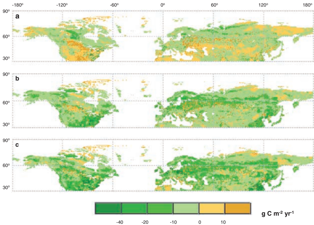
Fig. 6. The spatial distribution of NCE simulated by TEM 5.0 for the periods 1920–1957 (a), 1958–1995 (b) and 1980–1995 (c). Positive values of NCE represent sources of CO 2 to the atmosphere, while negative values represent sinks of CO 2 into terrestrial ecosystems.
