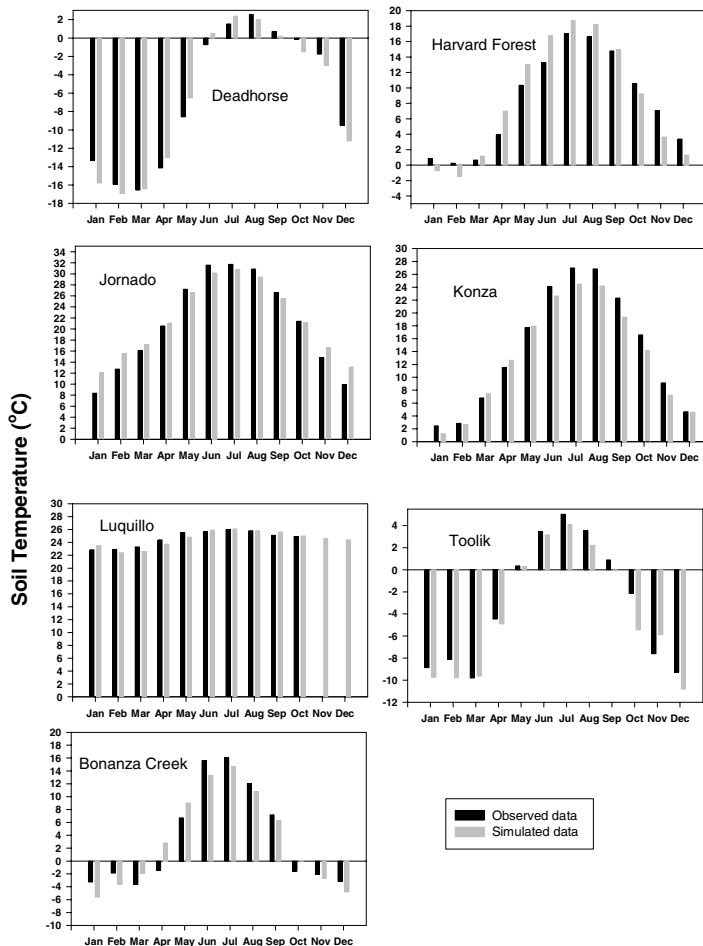
Fig. 2. Comparisons of monthly soil temperatures between observations and simulations by TEM 5.0. The temperatures were compared at 20 cm soil depth for the Deadhorse, Bonanza Creek, Harvard Forest and the Toolik sites, at 5 cm soil depth for the Jornada site, at 15 cm depth for the Luquillo site, and at 25 cm depth for the Konza site. For the descriptions of these sites see Table 2.
