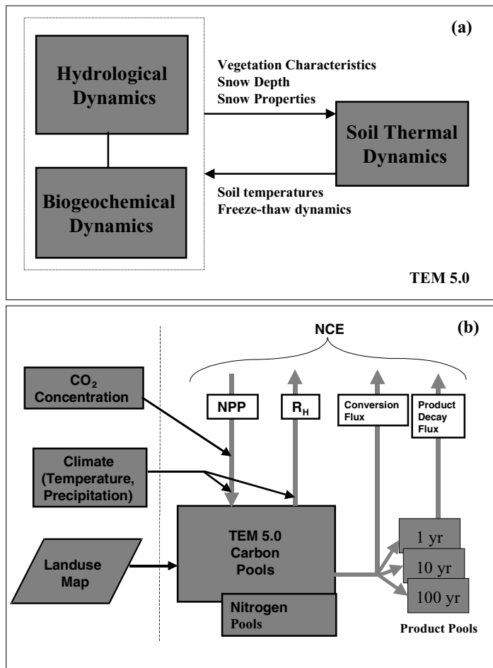
Fig. 1. (a) The structure of TEM 5.0 includes (1) hydrological dynamics based on a Water Balance Model (WBM, Vorosmarty et al., 1989), biogeochemistry dynamics based on the Terrestrial Ecosystem Model (TEM 4.2, McGuire et al., 2001), and soil thermal dynamics based on the Soil Thermal Module (STM, Zhuang et al., 2001). Among the three components, the STM receives vegetation characteristics from TEM, receives snow depth and snow properties from the WBM, and provides simulated soil temperatures and freeze-thaw dynamics to TEM to drive ecosystem processes. (b) Overview of the simulation protocol implemented by TEM 5.0 in this study to assess the concurrent effects of increasing atmospheric CO 2 , climate variability, and cropland establishment and abandonment during the 20th century.
