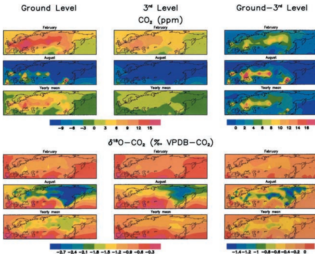
Fig. 7. Rectification gradients of \text{CO}_2 and \delta^{18}\text{O}-\text{CO}_2 at ground (first column) and third (second column) level of the model, approximately 30 and 800 m respectively, above ground. The third column is the difference between the first and second column. In the third column, the colour bar differs from those used in columns one and two. We suppressed longitude and latitude labelling to make the plot intelligible. Longitude ranges from 15 to 170°W (–15 to 190°) and latitude ranges from 35 to 75°N. We subtracted the global mean concentration from each grid point as a reference. This gives negative values everywhere in \delta^{18}\text{O}-\text{CO}_2 over Eurasia because of the simulated strong north–south gradient.
