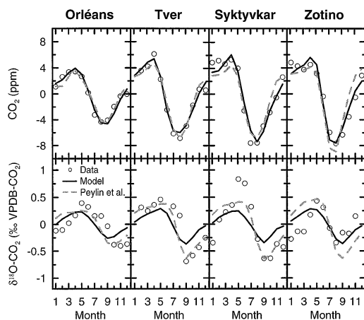
Fig. 6. Measured and modelled mean seasonal cycle of CO 2 and \delta^{18}\text{O}\text{-CO}_2 at Orléans, Tver, Syktyvkar, and Zotino at 3000 m a.s.l. Note that the data of Tver is not at 3000 m but a mean seasonal cycle extracted from flights above the atmospheric boundary layer (ABL).
