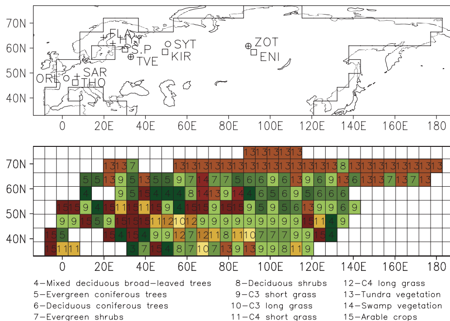
Fig. 2. Two different representations of the investigation area. In the upper frame are indicated the measurement stations of water isotopes (squares), \text{CO}_2 fluxes (cross) and atmospheric \text{CO}_2 with isotopes (circles) (ORL, Orléans; THO, Thonon-Bains; SAR, Sarrebourg; FLA, Flakaliden; HYY, Hyytiälä; S.P, St. Petersburg; TVE, Tver; SYT, Syktyvkar; KIR, Kirov; ZOT, Zotino; ENI, Enisejsk). In the lower frame, the boxes are the grids of the model and the colours with numbers stand for each vegetation class used (4–15 of 23 overall in the model).
