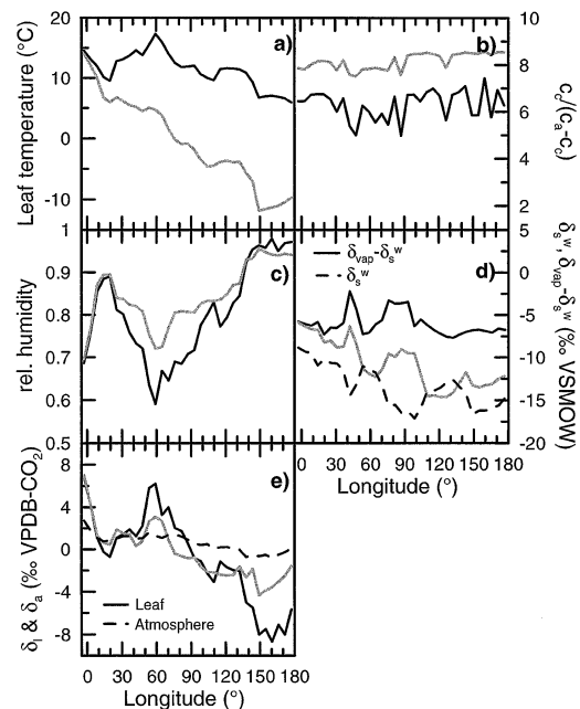
Fig. 10. Variables which determine the \delta^{18}\text{O}\text{-CO}_2 discrimination of assimilation. Black lines are assimilation-weighted values, and grey lines are not assimilation-weighted (see text for the difference between assimilation-weighted or not).
