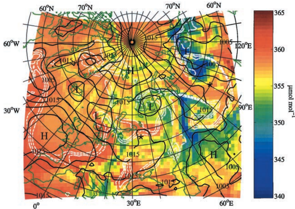
Fig. 4. Instantaneous \text{CO}_2 mixing ratios (given in \mu\text{mol mol}^{-1} ) at 12.00 UTC 24 July 1998 as calculated by MATCH in model level eight corresponding to approximately 770 hPa. Also shown is the surface pressure (hPa) reduced to mean sea level (full black lines) and a selection of equivalent potential temperatures (312, 315, and 318 K) at model level eight (dashed white lines). Stars denote the location of the EURO-SIB stations Zotino and Fyodorovskoye.
