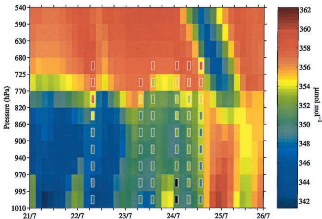
Fig. 6. Simulated time-series of vertical profiles of CO 2 at Zotino (60.5°N, 89.4°E) during the period 00.00 UTC 21 July until 00.00 UTC 26 July 1998. Observed profiles (Lloyd et al., 2002) averaged in vertical bins corresponding to the model grid are included in white frames using the same colour scale (black denotes higher mixing ratios than on the colour scale). Unit: \mu\text{mol mol}^{-1} .
