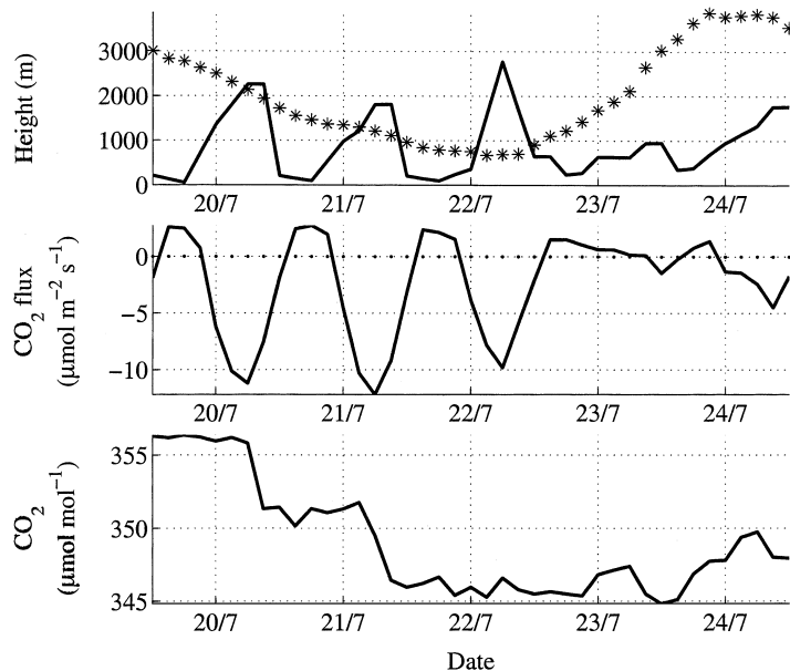
Fig. 8. The upper panel shows vertical path of the trajectory arriving at 600 hPa above Zotino (60.5°N, 89.4°E) at 12.00 UTC 24 July 1998 (*) and the boundary layer height as calculated by MATCH for the gridboxes closest to the path of the trajectory (full line). The middle panel shows the surface flux of CO 2 in the gridboxes closest to the trajectory (unit: \mu\text{mol m}^{-2} \text{s}^{-1} ). The lower panel shows CO 2 mixing ratios calculated by MATCH in the gridboxes closest to the trajectory vertically interpolated to the height of the trajectory (unit: \mu\text{mol mol}^{-1} ).
