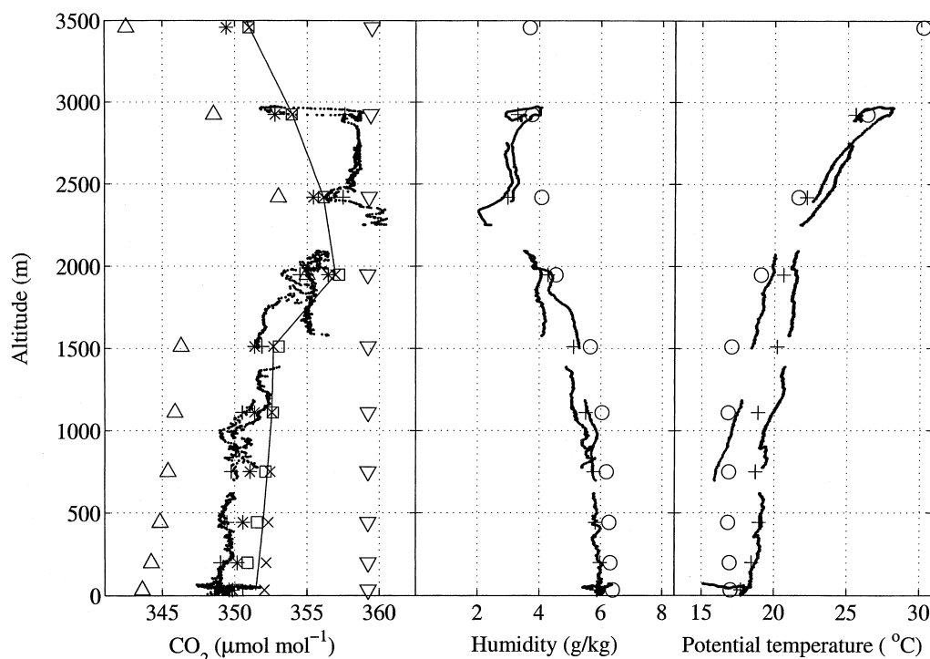
Fig. 10. Vertical profiles of CO 2 ( \mu\text{mol mol}^{-1} ), specific humidity ( \text{g kg}^{-1} ) and potential temperature ( ^{\circ}\text{C} ) at Zotino ( 60.5^{\circ}\text{N} , 89.4^{\circ}\text{E} ) at 12.00 UTC 24 July 1998: (●) Observations (Lloyd et al., 2002); (+) averages of the observations in layers corresponding to the model levels; (○) ECMWF data for humidity and temperature. CO 2 profiles are from simulations with (—) the reference case, (▽) no internal sources, (△) terrestrial surface fluxes increased by 100%, (*) surface fluxes increased by 20%, (□) the degree of mixing in the PBL reduced to 50% and (×) the degree of mixing in the PBL increased with 100%.
