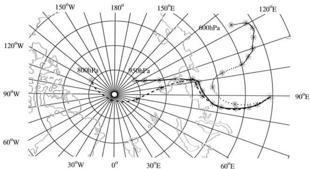
Fig. 7. Three-dimensional 5-d back trajectories arriving at different pressure levels at Zotino (60.5°N, 89.4°E) at 12.00 UTC 24 July 1998. Stars denote positions of trajectories every 12 h.
