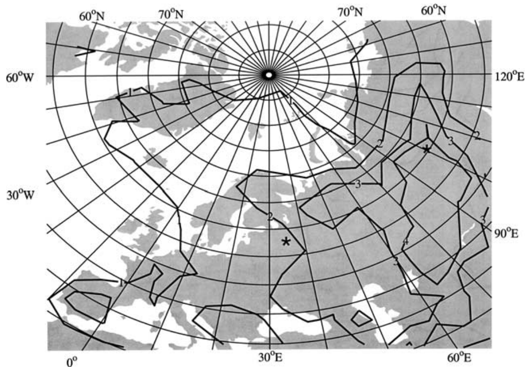
Fig. 11. Signal-to-noise ratio (SNR) at model level five (approximately 900 hPa) for July 1998. The SNR is calculated as the difference between the reference simulation including terrestrial sources/sinks and a simulation without, divided by the standard deviation of the run including the terrestrial sources/sinks. Stars denote the location of the EUROSIB stations Zotino and Fyodorovskoye. Isolines are 1, 2, 3, and 4.
