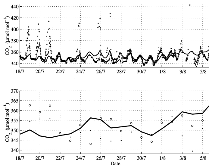
Fig. 5. Surface mixing ratios of CO 2 at Zotino (60.5°N, 89.4°E) during the period 00.00 UTC 18 July until 00.00 UTC 6 August 1998. The full line shows the calculated mixing ratios at the lowest model level, dotted lines are observed data from the forest and circles observed data from the bog (Styles et al., 2002; Arneth et al., 2002). The upper panel shows the full diurnal cycle, the lower panel shows diurnally averaged mixing ratios.
