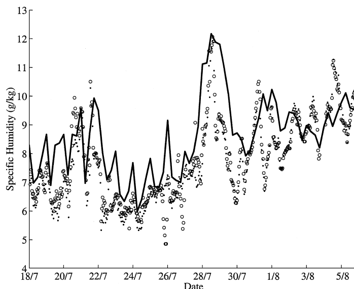
Fig. 1. Specific humidity at Zotino ( 60.5^\circ\text{N} , 89.4^\circ\text{E} ) during the period 00.00 UTC 18 July until 00.00 UTC 6 August 1998. The full line is data from ECMWF interpolated to the rotated 1^\circ \times 1^\circ grid used by MATCH. Data are from the lowest model level, about 30 m above the ground. Observed data from the forest (dotted) and the bog (circles) are also shown (Tchekobokova et al., 2002; Kurbatova et al., 2002).
