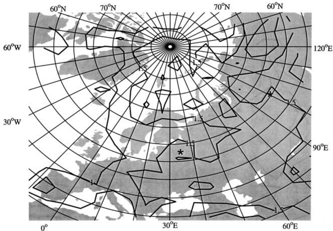
Fig. 12. As Fig. 11, but for August 1998. Isolines are 1, 1.5, and 2.
