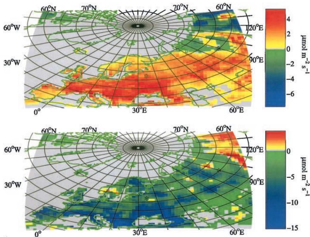
Fig. 2. Net flux of \text{CO}_2 on 24 July as calculated by the TURC model with the addition of the diurnal cycle described in the text. Conditions are shown at 00.00 UTC (upper panel) and 12.00 UTC (lower panel). Stars denote the location of the EUROSIB stations Zotino and Fyodorovskoye. Positive values indicate a \text{CO}_2 flux to the atmosphere. Unit: \mu\text{mol m}^{-2} \text{s}^{-1} .
