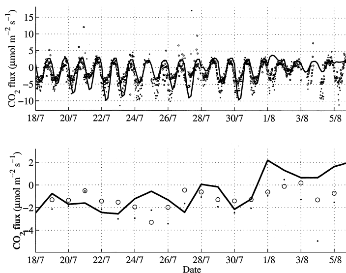
Fig. 3. Surface flux of CO 2 at Zotino (60.5°N, 89.4°E) during the period 00.00 UTC 18 July until 00.00 UTC 6 August 1998. The full line shows the calculated fluxes, dotted lines are observed data from the forest and circles data from the bog (Styles et al., 2002; Arneeth et al., 2002). The upper panel shows instantaneous data every 3 h; the lower panel shows diurnally averaged values.
