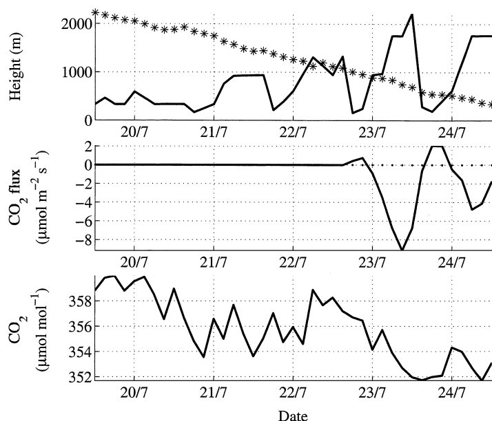
Fig. 9. As Fig. 8, but for the trajectory arriving at 950 hPa.
