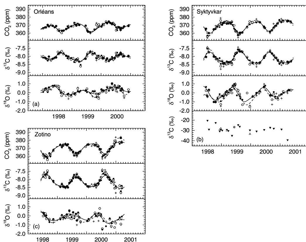
Fig. 2. (a) CO 2 mixing ratio, δ 13 C–CO 2 and δ 18 O–CO 2 observed in aircraft samples over Orléans, France (1°E, 48°N) at three height levels, 2000 m (crosses), 2500 m (open circles) and 3000 m (closed circles). Dashed lines are harmonic fit curves through the 2000 m data, solid lines harmonic fit curves through the 3000 m data. (b) Same as (a) but for the Russian site Syktyvkar (52°E, 61°N). The lowest panel shows apparent source signatures calculated from individual profiles where CO 2 gradients between 3000 m and 2000 m (closed symbols) and 2500 m (open symbols) were larger than 1 ppm. (c) Same as (a) but for the Siberian site Zotino (89°E, 61°N).
