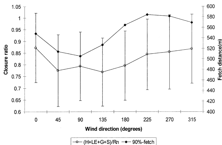
Fig. 2. Energy balance closure ratio (H + \lambda E + G + S)/R_n and fetch distance plotted against wind direction bin-averaged for each 45^\circ for the 1999 growing season. Error bars are one standard deviation.
