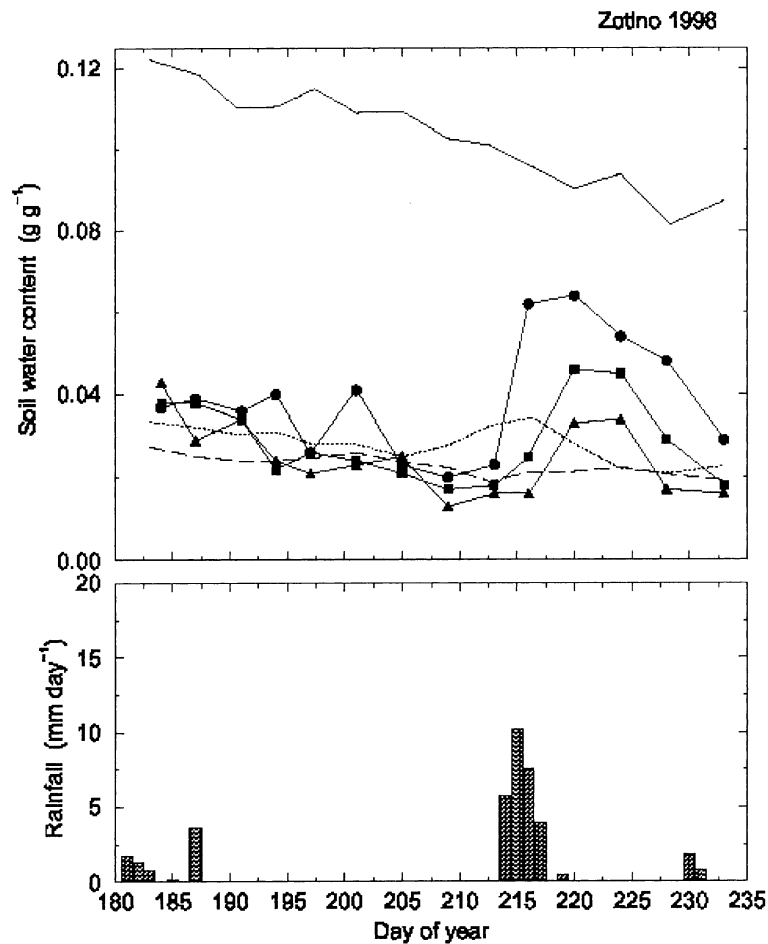
Fig. 7. Variation in soil water content and daily precipitation during summer 1998. (●) 0–0.1 m depth; (■) 0.1–0.2 m depth; (▲) 0.2–0.3 m depth; (---) 0.6–0.7 m depth; (.....) 0.9–1.0 m depth; (—) 1.9–2.0 m depth. Due to greater heterogeneity in soil physical properties and water content at depths below 0.5 m, three-point running averages of the original data are shown for lower depth samples for increased clarity of presentation.
