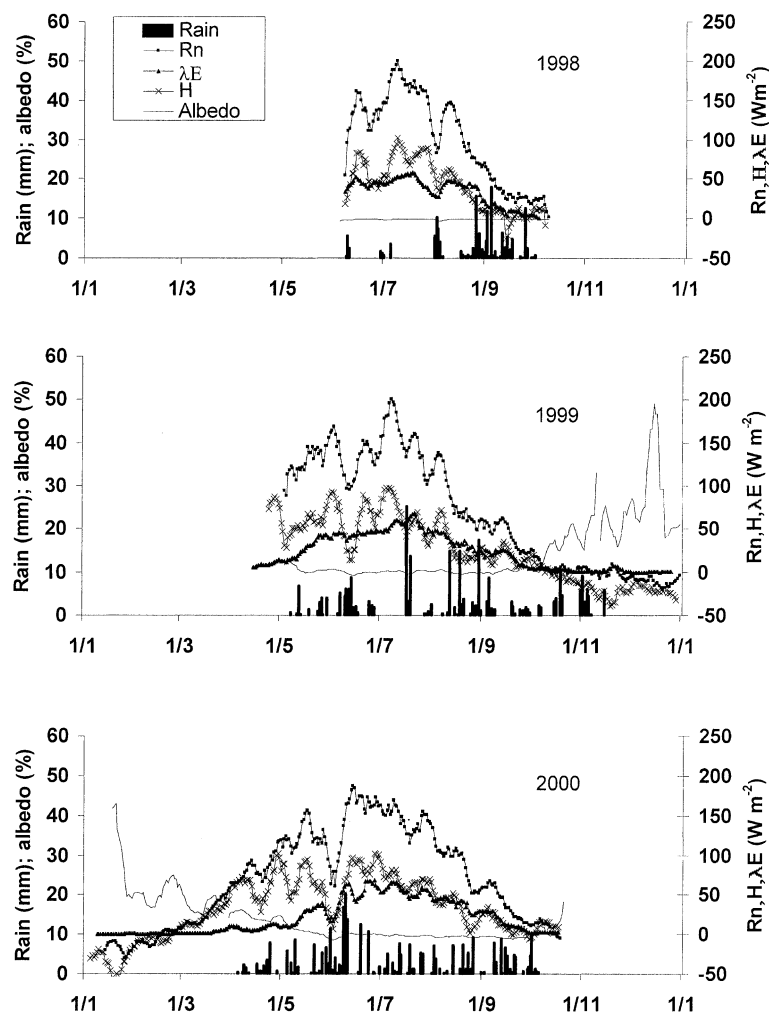
Fig. 3. Seven-day running averages of daily albedo, net radiation ( R_n ), latent heat ( \lambda E ), sensible heat ( H ) and daily precipitation (not smoothed) for 1998–2000.
