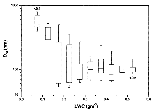
Fig. 5. Activation diameter (10 th , 25 th , median, 75 th , 90 th percentile) versus LWC classes for the whole measuring campaign for stable cloud times ( LWC 15 th percentile > 0.02 \text{ g m}^{-3} ).
