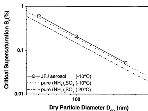
Fig. 8. Critical supersaturation for JFJ aerosol at ambient temperature, and ammonium sulfate at -10 and 20^\circ\text{C} calculated with the model from (Brechtel and Kreidenweis, 2000a).
