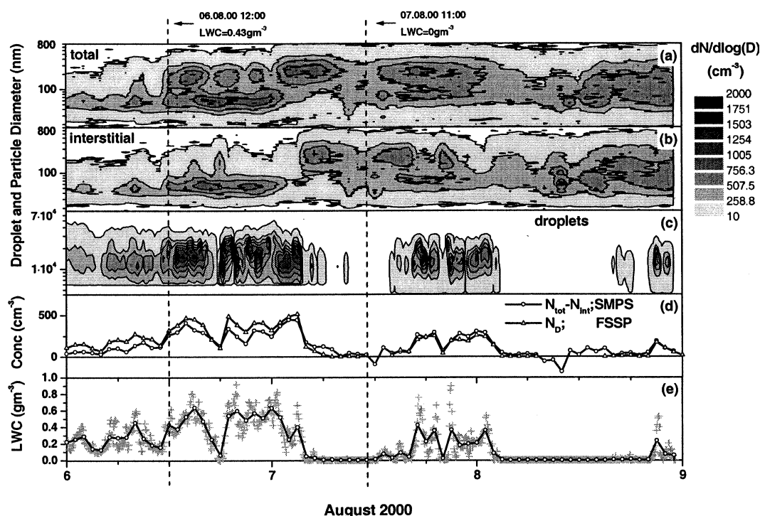
Fig. 1. Contour plots of the total (a) and interstitial (b) aerosol size distributions, droplet size distribution (c), droplet number concentration and the difference between total and interstitial aerosol number concentration (d), and the liquid water content of the ambient air (e). The presented data for the period 6–9 August 2000 0:00 LST are 1-h averages (a, b, d, e), 20-min averages (c), while the crosses in (e) are 5-min values.
