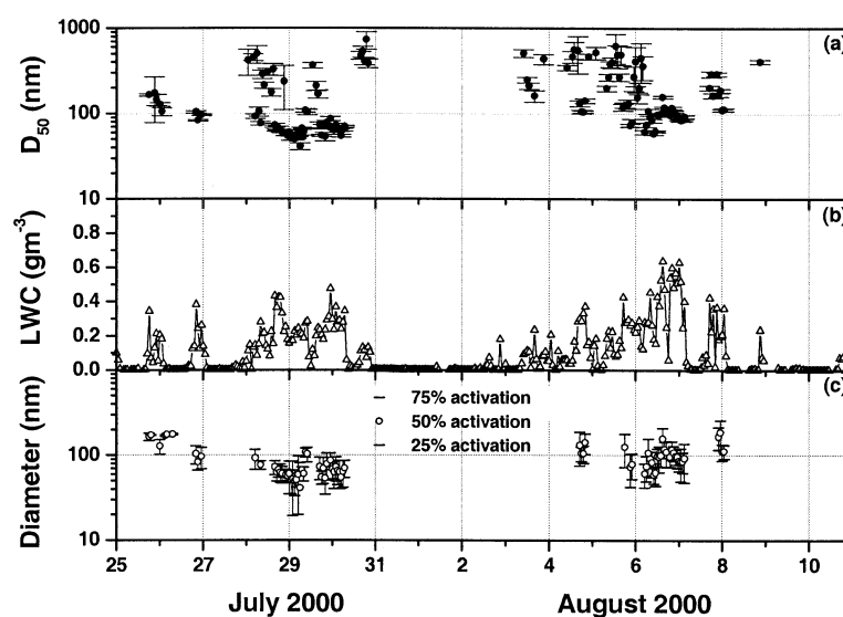
Fig. 4. Diameter of 50% scavenging (a) in comparison with the liquid water content (b) over the whole measuring period. As parameter of the steepness of the activation the diameters of 25% and 75% activation are added as bars (c). The activation diameter is only plotted for LWC 15 th percentile > 0.02 \text{ g m}^{-3} .
