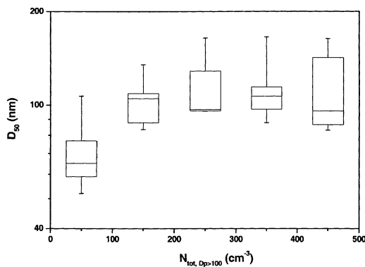
Fig. 6. Diameter of 50% activation (10 th , 25 th , median, 75 th , 90 th percentile) plotted versus total number concentration of particles with a diameter greater than 100 nm. Only activation diameters for 15 th percentile of LWC higher than 0.02 g m -3 were used for calculation.
