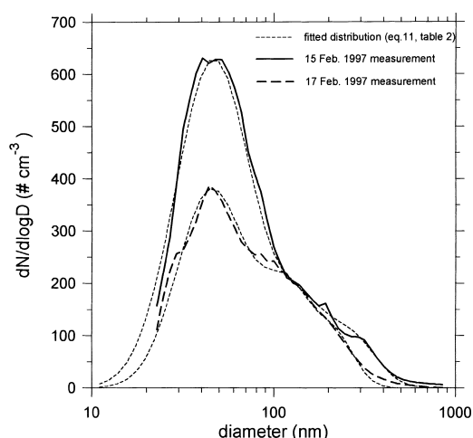
Fig. 3. Measured number density distribution functions for aerosol particles for the 15 February 1997 (solid curve) and 17 February 1997 (dashed curve). The dotted curves give the number density distribution function of aerosol particles resulting from eq. (11) and Table 2.
