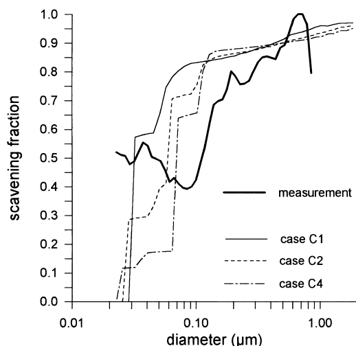
Fig. 7. Scavenging fraction as a function of dry aerosol particle diameter. The fat solid curve gives the measurements from 15 February at 11:00 LT. The thin curves represent the results from the cases C1, C2 and C4 as detailed in Table 6 considering homogeneous entrainment.
