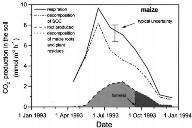
Fig. 5. Monthly means of the different sources of soil produced CO 2 for maize (Weiherbach sampling site 1, 1993). After harvest, the \delta^{13}\text{C} signal of C4-plants in the maize field was interpreted as microbial decomposition of plant residues and dead roots.
