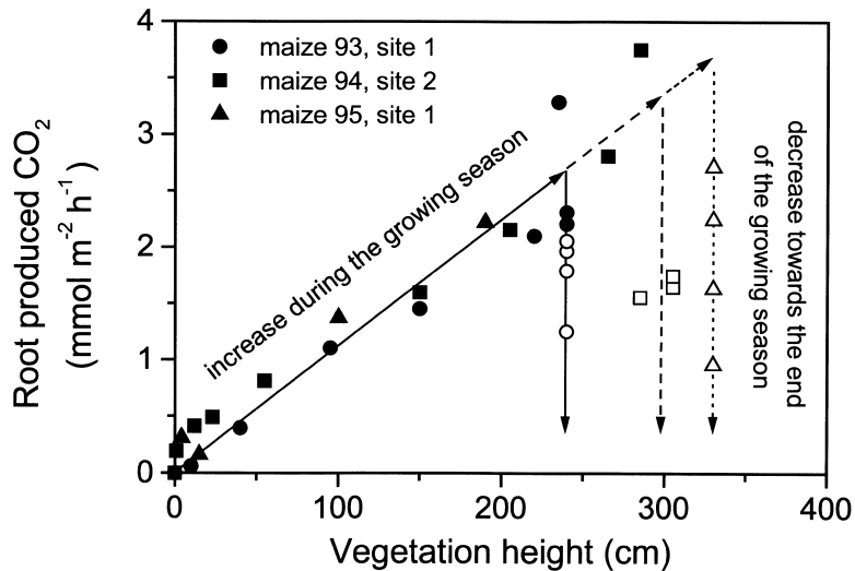
Fig. 3. Correlation between vegetation height and root-produced \text{CO}_2 for maize (linear regression: R^2 \geq 0.88 ). The same slope was observed for all 3 years. Values obtained at the end of the respective growing season are shown as open symbols. At this time, lower plant activity resulted in smaller amounts of root-produced \text{CO}_2 .
