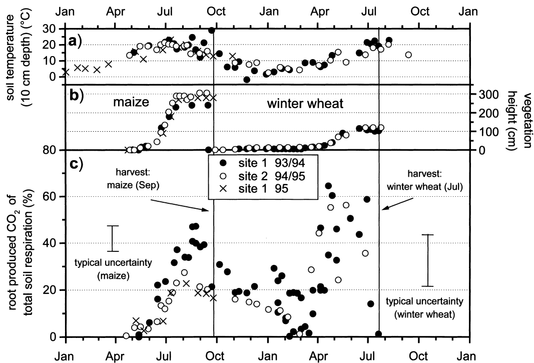
Fig. 2. Combined results for the Weiherbach sampling sites 1 and 2 of (a) soil temperature (10 cm depth), (b) vegetation height and (c) the percentage of root-produced \text{CO}_2 for one 2-year crop rotation period. The vertical lines indicate the time of the harvest.
