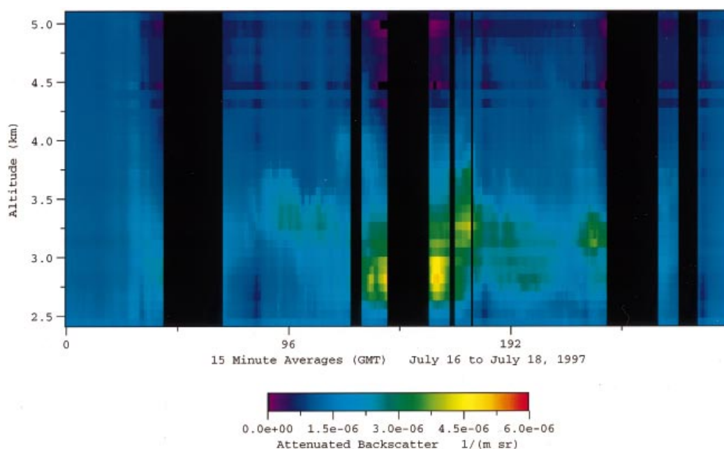
Fig. 7. 3-day attenuated backscatter signal (ABS) (\text{m sr})^{-1} time series from 16 through 18 July 1997. ABS values have an average error of 5% and each ABS profile is a 15-min average (GMT). The black gaps represent periods when the MPL was not oriented in the vertical mode.
