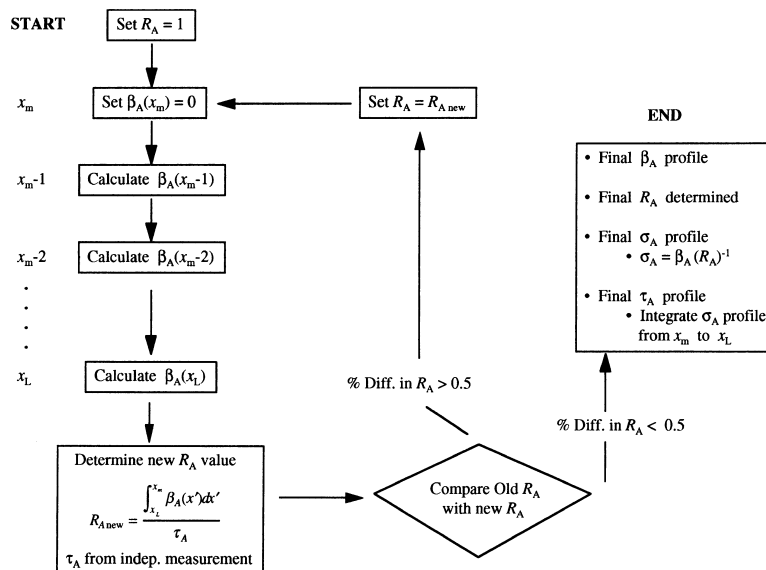
Fig. 12. Schematic representation of the lidar inversion algorithm.
