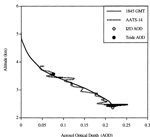
Fig. 10. Lidar aerosol optical depth (AOD) profile (average error \pm 0.013 ) at 18:45 GMT on 17 July 1997 (solid line). The calculated columnar backscatter-extinction ratio ( \text{sr}^{-1} ) is 0.027 \pm 0.007 . The AOD profile measured with AATS-14 from 18:30 to 18:45 GMT, and the AOD measured by the IZO Cimel and the Teide shadowband, are also shown. Errors in the AOD from the other instruments are \pm 0.01 or less.
