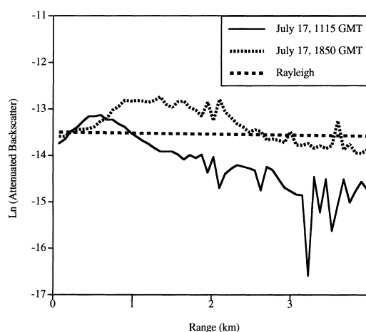
Fig. 11. Horizontal lidar profiles of the natural logarithm of the attenuated backscatter signal ( \text{m sr}^{-1} ). ABS values have an average of 5% error. A 15-min average horizontal profile at 11:15 GMT and a 5-min average horizontal profile at 18:50 GMT on 17 July are shown along with a calculated Rayleigh horizontal profile for the IZO altitude.
