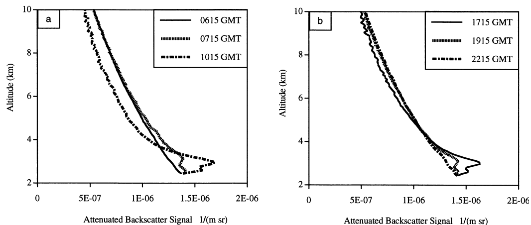
Fig. 5. (a) Attenuated backscatter signals (\text{m sr})^{-1} in the morning of 29 June 1997. (b) Attenuated backscatter signals (\text{m sr})^{-1} in the afternoon on 29 June 1997. The values have less than 5% error and each profile is a 15-min average, starting 15 min prior to the time shown.
