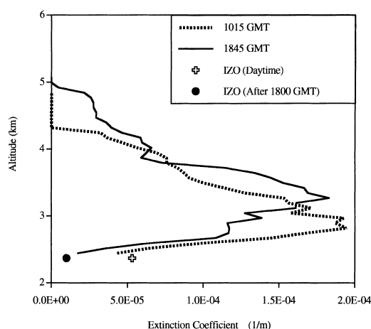
Fig. 9. Lidar aerosol extinction coefficient ( \text{m}^{-1} ) profiles ( \sim 7\% error) at 10:15 and 18:45 GMT on 17 July 1997. The columnar AOD ( \pm 0.01 ) for each profile is 0.205 and 0.217 respectively. The calculated columnar backscatter–extinction ratios ( \text{sr}^{-1} ) for each profile are 0.048 \pm 0.012 and 0.027 \pm 0.007 respectively. The average aerosol extinction coefficients obtained at IZO ( \pm 5.5 \times 10^{-7} ) from 07:00 to 18:00 GMT (daytime) and after 18:00 GMT are also shown.
