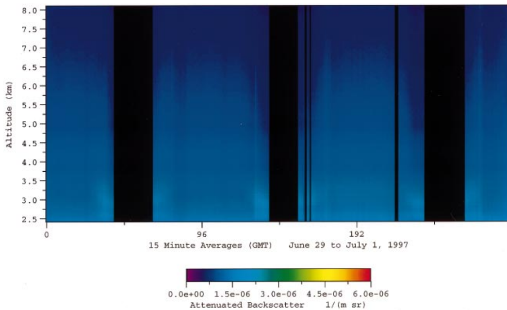
Fig. 4. 3-day attenuated backscatter signal (ABS) (\text{m sr})^{-1} time series from 29 June through 1 July 1997. ABS values have less than 5% error and each ABS profile is a 15-min average (GMT). The black gaps represent periods when the MPL was not oriented in the vertical mode.
