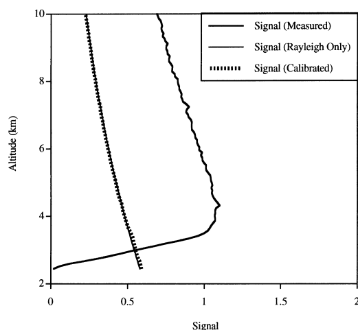
Fig. 3. The measured MPL signal, a calculated Rayleigh lidar signal, and the final calibrated MPL signal are shown for 00:00 GMT on 30 June 1997.
