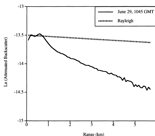
Fig. 6. Horizontal lidar profile of the natural logarithm of the attenuated backscatter signal (ABS) ( \text{m sr}^{-1} ). ABS values have less than 5% error. A 15-min average horizontal profile at 10:45 GMT on 29 June is shown along with a calculated Rayleigh horizontal profile for the IZO altitude.
