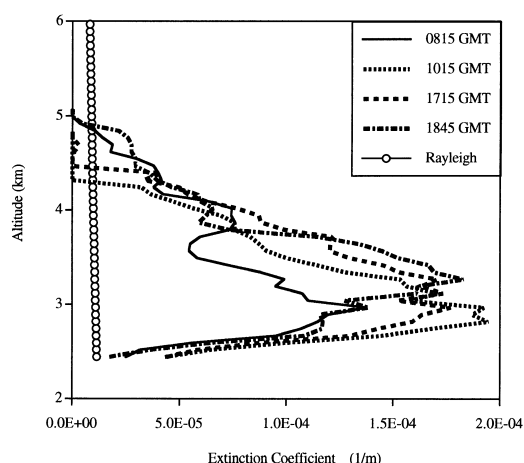
Fig. 8. Lidar aerosol extinction coefficient ( \text{m}^{-1} ) profiles ( \sim 7\% error) at 08:15, 10:15, 17:15, and 18:45 GMT on 17 July 1997. The columnar AOD ( \pm 0.01 ) for each profile is 0.161, 0.205, 0.226, and 0.217 respectively. The calculated columnar backscatter–extinction ratios ( \text{sr}^{-1} ) for each profile are 0.026 \pm 0.007 , 0.048 \pm 0.012 , 0.073 \pm 0.018 , and 0.027 \pm 0.007 respectively. The Rayleigh extinction coefficient profile is shown for comparison.
