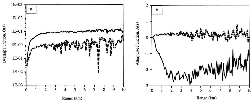
Fig. 2. (a) Overlap functions, O(z) , calculated on 29 June (solid line) and 15 July (dotted line) 1997. (b) Afterpulse functions, A(z) , calculated on 29 June (solid line) and 15 July (dotted line) 1997.
