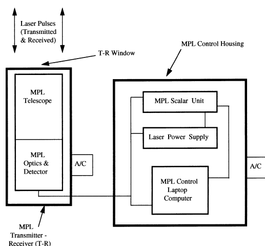
Fig. 1. Schematic diagram of the micro-pulse lidar system (not to scale).
