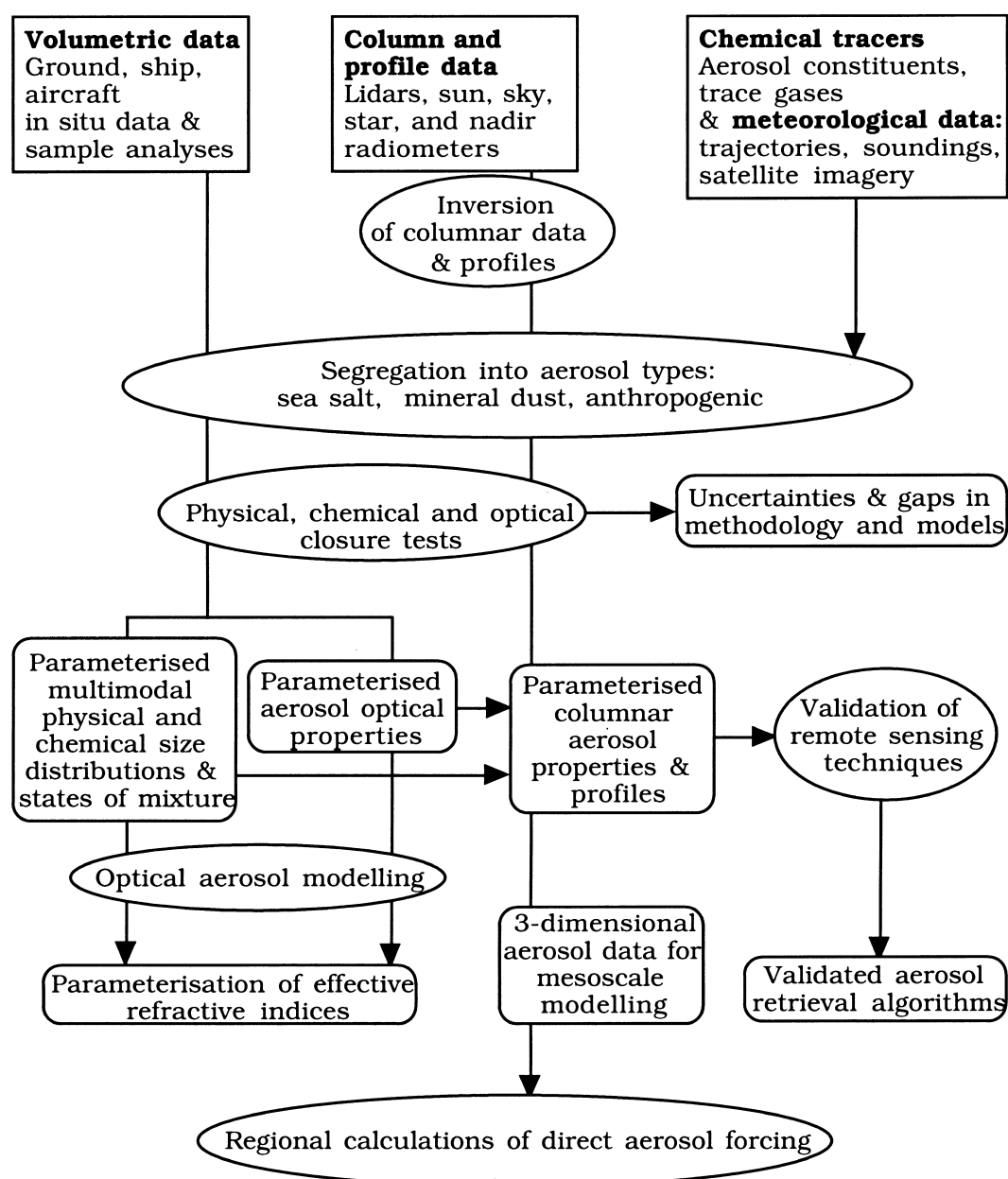
Fig. 2. Flow chart of the evaluation methodology of CLEARCOLUMN. Squares mark input data. Ovals stand for processing steps and rounded rectangles indicate deliverables.
