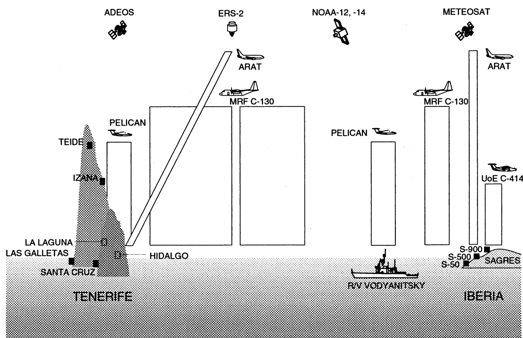
Fig. 1. Schematic overview of CLEARCOLUMN sites and platforms.
