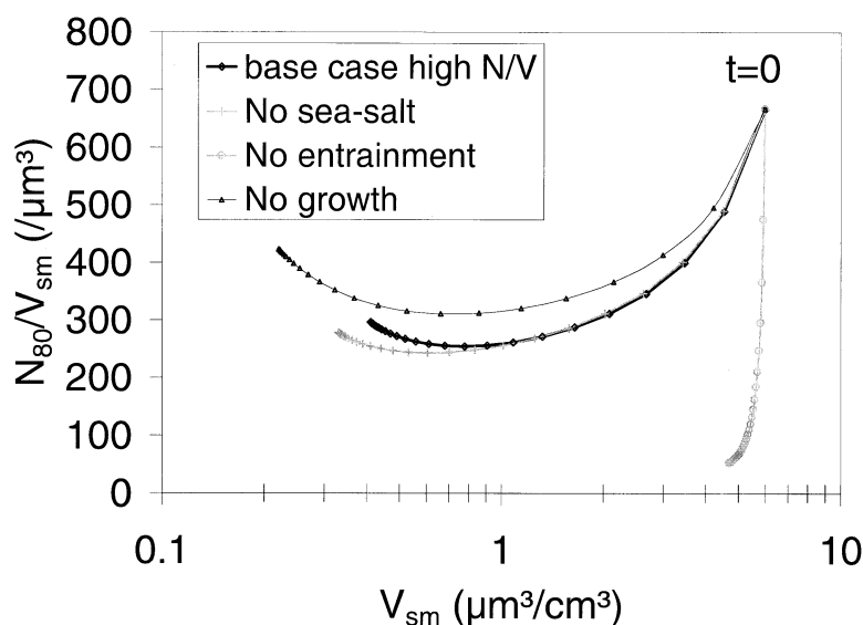
Fig. 4. Effect of various processes on the N_{80}/V_{sm} ratio as function of V_{sm} from the analytical model (case 2 only). Symbols indicate 12-h intervals when the aerosol evolves from high to low V_{sm} over 14 days transport in the MBL. Results are similar for case 1.
