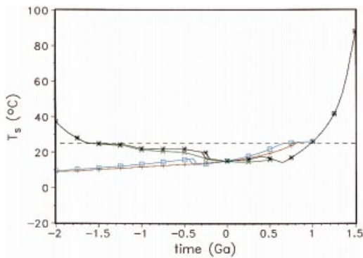
Fig. 2. Past and future variation of the mean global surface temperature T_s(t) for the four employed models: GSM-asymptotic (+), GDM-asymptotic (x), GSM-parabolic (□), and GDM-parabolic (*). The two parabolic models have multiple solutions in the past. The horizontal dashed line indicates the “optimal” biogeophysical temperature, i.e., 25°C.
