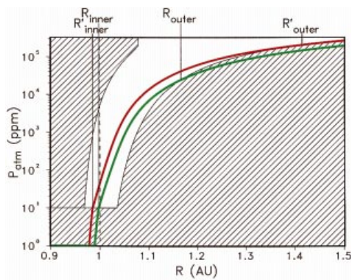
Fig. 7. The habitable zone (non-dashed region) for an earth-like planet in the "near" future (0.5 Ga). For GDM-asymptotic (green line) the respective boundaries are R_{\text{inner}} = 1.0 AU and R_{\text{outer}} = 1.17 AU. Because R_{\text{inner}} will exactly coincide with the actual distance of planet earth from the sun (1 AU), the life span of the biosphere will end at this time. For GSM-asymptotic (red line) the respective boundaries are R'_{\text{inner}} = 0.99 AU and R'_{\text{outer}} = 1.41 AU.
