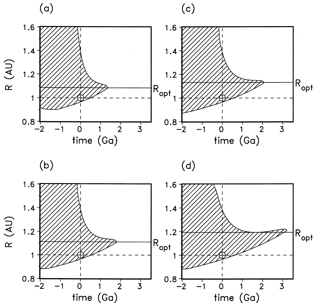
Fig. 10. Habitable zones of the GDM-asymptotic for the four alternative continental-growth models: (a) delayed growth, (b) linear growth, (c) Reymer and Schubert, (d) constant area. Obviously, the so-calculated HZs do not differ in their qualitative behaviour. The biosphere life span varies only slightly in magnitude and is always shorter than in the geostatic case (GSM). Exact values for the biosphere life span, the optimum distance, and the maximum life span, respectively, can be found in Table 1.
