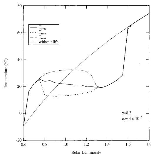
Fig. 5. Stabilization of mean planetary temperature over range of solar luminosity L at c_p = 3 \times 10^{13} , \gamma = 0.3 . The maximum and minimum temperatures shown reflect the amplitude of the temperature oscillations. All averages, maxima, and minima are computed over a 1000 year period after first initializing the model for 1200 years. The dotted line shows temperature without life, i.e., at a constant value of A = 0.5 .
