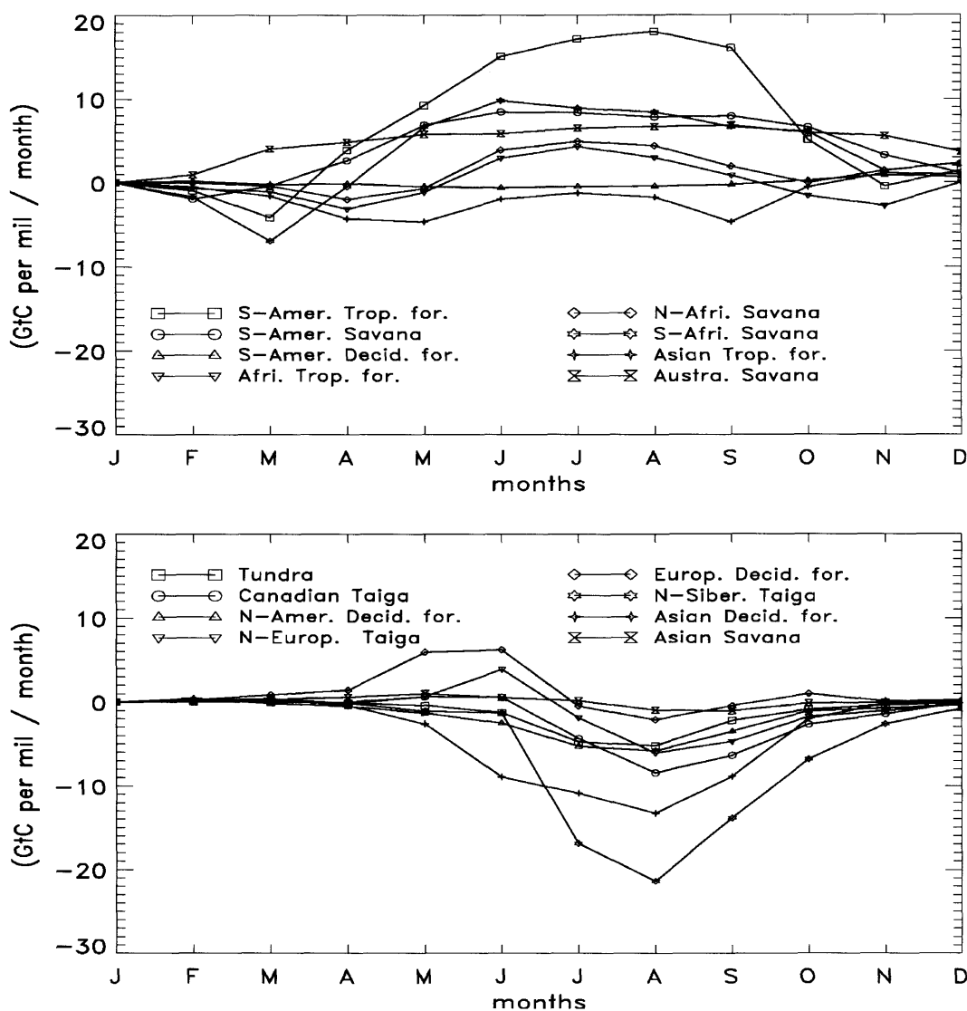
Fig. 8. Seasonal variations of the flux of \delta^{18}\text{O} in atmospheric \text{CO}_2 (in \text{GtC‰ month}^{-1} ) from 16 land ecosystems (Fig. 5), before atmospheric transport. Values represent the overall contribution of photosynthesis and respiration ( A\Delta_A + F_{\text{resp}}\Delta_R , eq. (A3)). All curves are shifted to zero in January as we will only discuss the seasonality of the fluxes.
