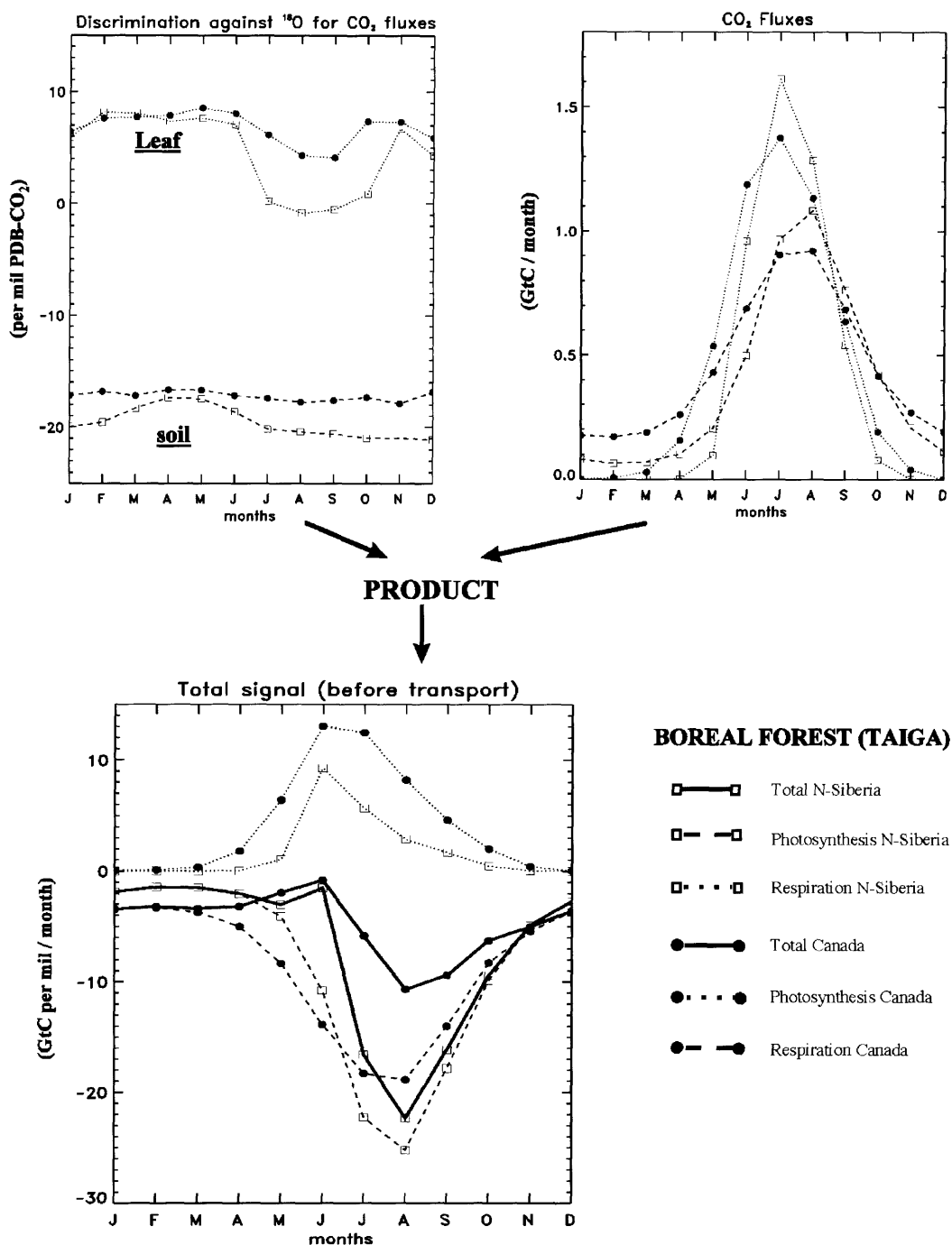
Fig. 9. Seasonal variations of the flux of \delta^{18}\text{O} in atmospheric \text{CO}_2 (in GtC % month ^{-1} , lower graph) from the northern Siberian taiga and the Canadian taiga (regions 4 and 2, respectively, Fig. 5), before atmospheric transport. The overall contribution (solid lines) is the sum of the photosynthesis and respiration contributions ( A\Delta_A and F_{\text{resp}}\Delta_R , respectively, eq. (A3)), for each region. The isotopic signal from photosynthesis and respiration results from a product between the \text{CO}_2 flux (net assimilation and ecosystem respiration, respectively; upper right graph) and the discrimination against ^{18}\text{O} compared to ^{16}\text{O} associated with this flux (upper left graph).
