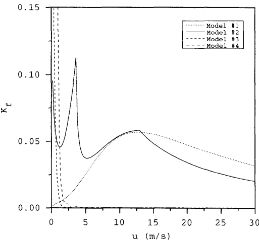
Fig. 9. K_f versus wind speed extrapolated for all capillary wave numbers. The models are tabulated in Table 2.
