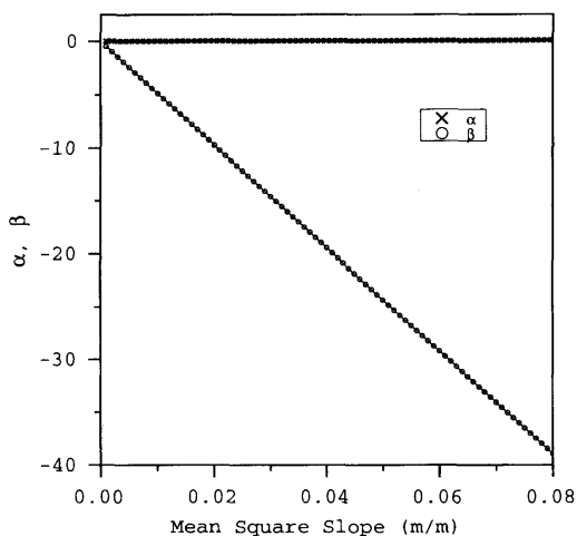
Fig. 5. Plot of \alpha and \beta versus \bar{S}^2 for the range of \bar{S}^2 presented in Fig. 1. The solid lines are obtained from eqs. (12) and (13).
