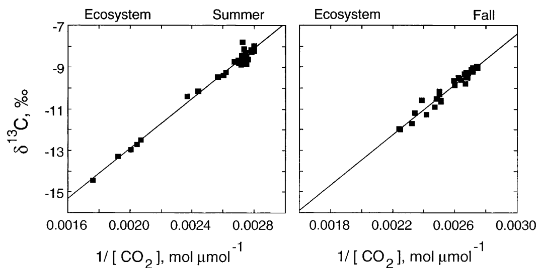
Fig. 6. Comparison of the relationships between 1/CO_2 concentration and the carbon isotope ratio of CO_2 in air samples collected from different heights above ground at night in a black spruce forest in Saskatchewan during the summer and fall 1996.
