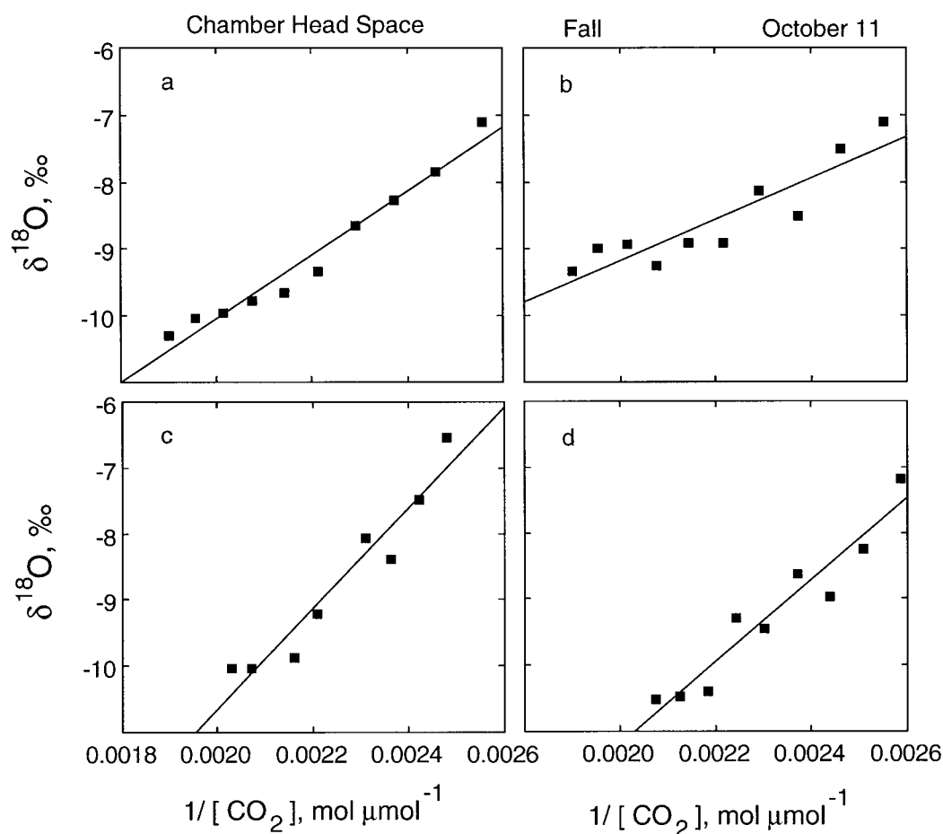
Fig. 10. Comparison of the relationships between 1/CO_2 concentration and the oxygen isotope ratio of CO_2 in air samples collected from moss/soil respiration chambers in a black spruce forest in Saskatchewan during 11 October 1996. Format of the figure is the same as that described in Fig. 3.
