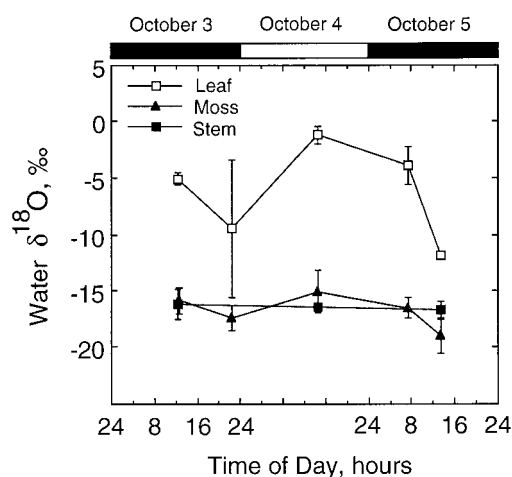
Fig. 8. Daily variation in the oxygen isotope ratio of water extracted from black spruce leaf and stem tissue, and moss tissue collected in a black spruce forest in Saskatchewan during fall 1996.
