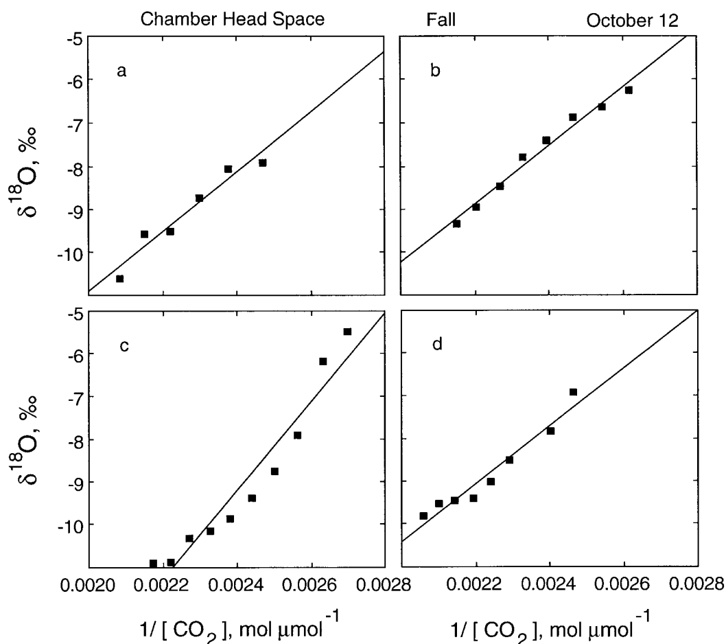
Fig. 11. Comparison of the relationships between 1/CO_2 concentration and the oxygen isotope ratio of CO_2 in air samples collected from moss/soil respiration chambers in a black spruce forest in Saskatchewan during 12 October 1996. Format of the figure is the same as that described in Fig. 3.
