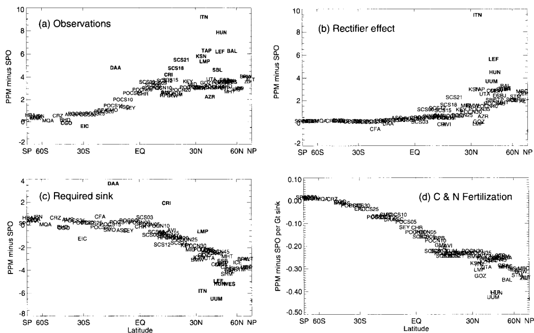
Fig. 1. Meridional profiles of annual mean CO 2 mole fraction at the locations of global view flask stations. The abscissae are scaled according to the sine of latitude, and the scales on the ordinate vary from panel to panel. The letter codes correspond to the station codes used for the stations in the global view data. Panel (a) shows observational data. Panels (b) through (d) show results for the final year of a 5 year tracer simulation in the CSU GCM. (b) is the result of a balanced biosphere using SiB2; (c) is the difference between the observations and the sum of fossil fuels + air-sea exchange + SiB2, indicating the required effect of a sink which balances the carbon budget and matches the annual profile of the data; (d) shows the effect of a 1 GtC/yr sink due to CO 2 fertilization and nitrogen deposition as simulated by SLAVE.
